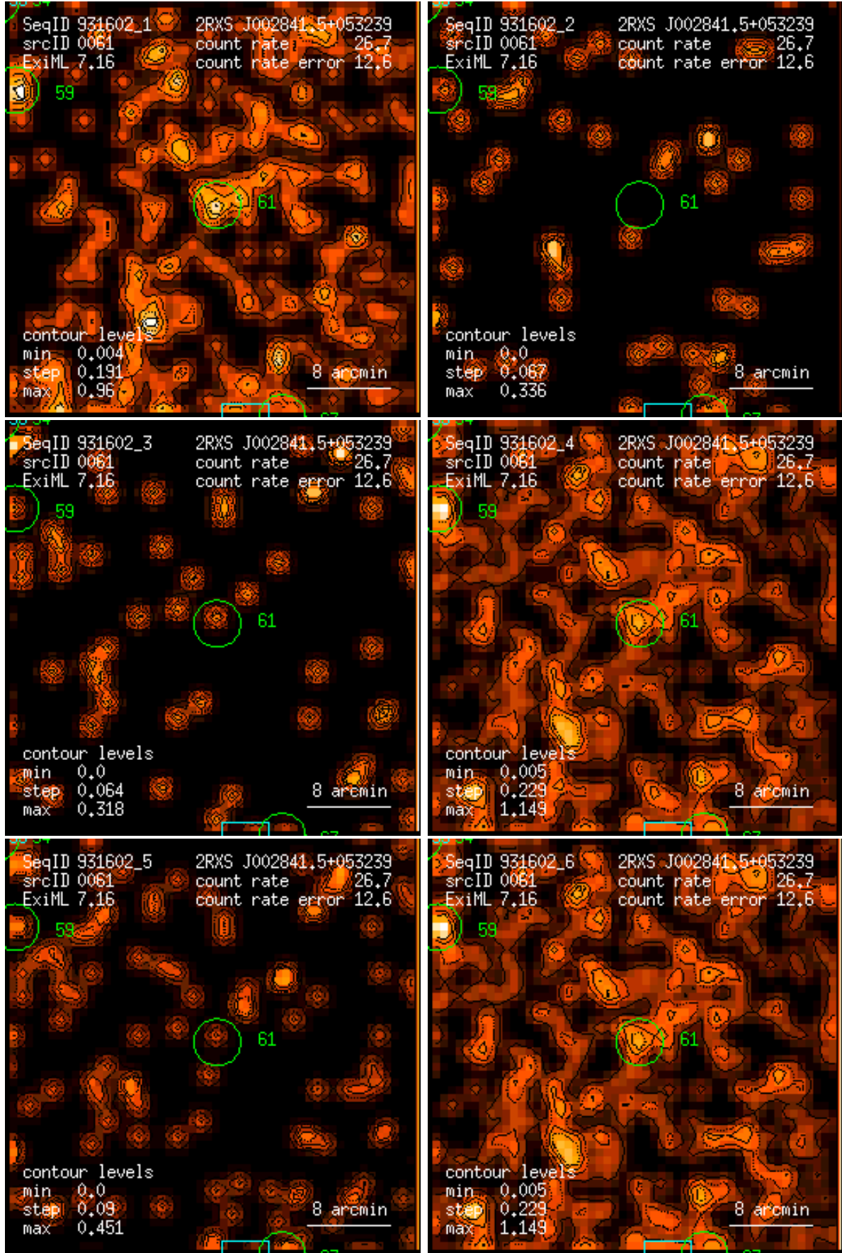
Figure 61: RASS 931602: detection 0061: band rate images, Gaussian filter: (1) PSPC channels 11 – 41, (2) 52 – 90, (3) 91 – 201, (4) 11 – 235, (5) 52 – 201, (6) 11 – 201. Broad band rates in counts/ks. Band rate contour levels in counts/ks/arcmin 2 .
