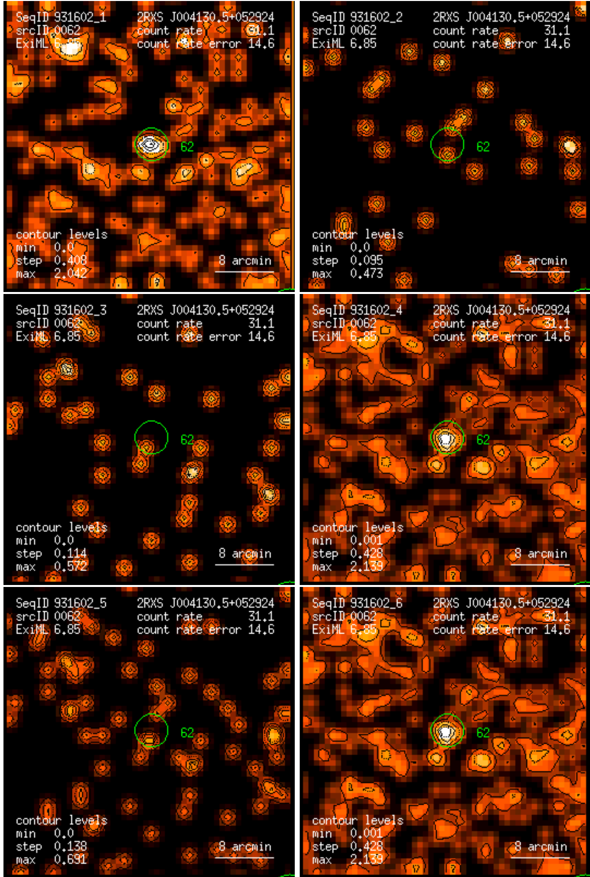
Figure 62: RASS 931602: detection 0062: band rate images, Gaussian filter: (1) PSPC channels 11 – 41, (2) 52 – 90, (3) 91 – 201, (4) 11 – 235, (5) 52 – 201, (6) 11 – 201. Broad band rates in counts/ks. Band rate contour levels in counts/ks/arcmin 2 .
