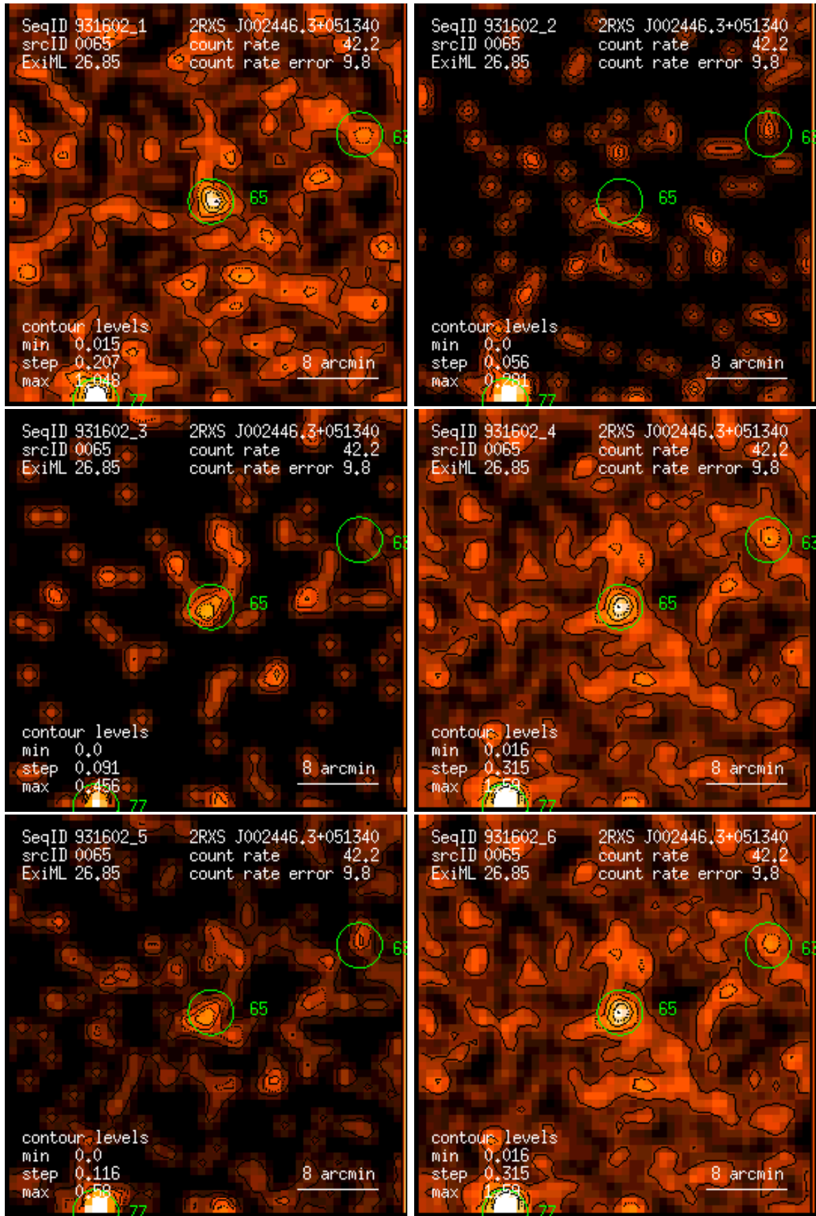
Figure 65: RASS 931602: detection 0065: band rate images, Gaussian filter: (1) PSPC channels 11 – 41, (2) 52 – 90, (3) 91 – 201, (4) 11 – 235, (5) 52 – 201, (6) 11 – 201. Broad band rates in counts/ks. Band rate contour levels in counts/ks/arcmin 2 .
