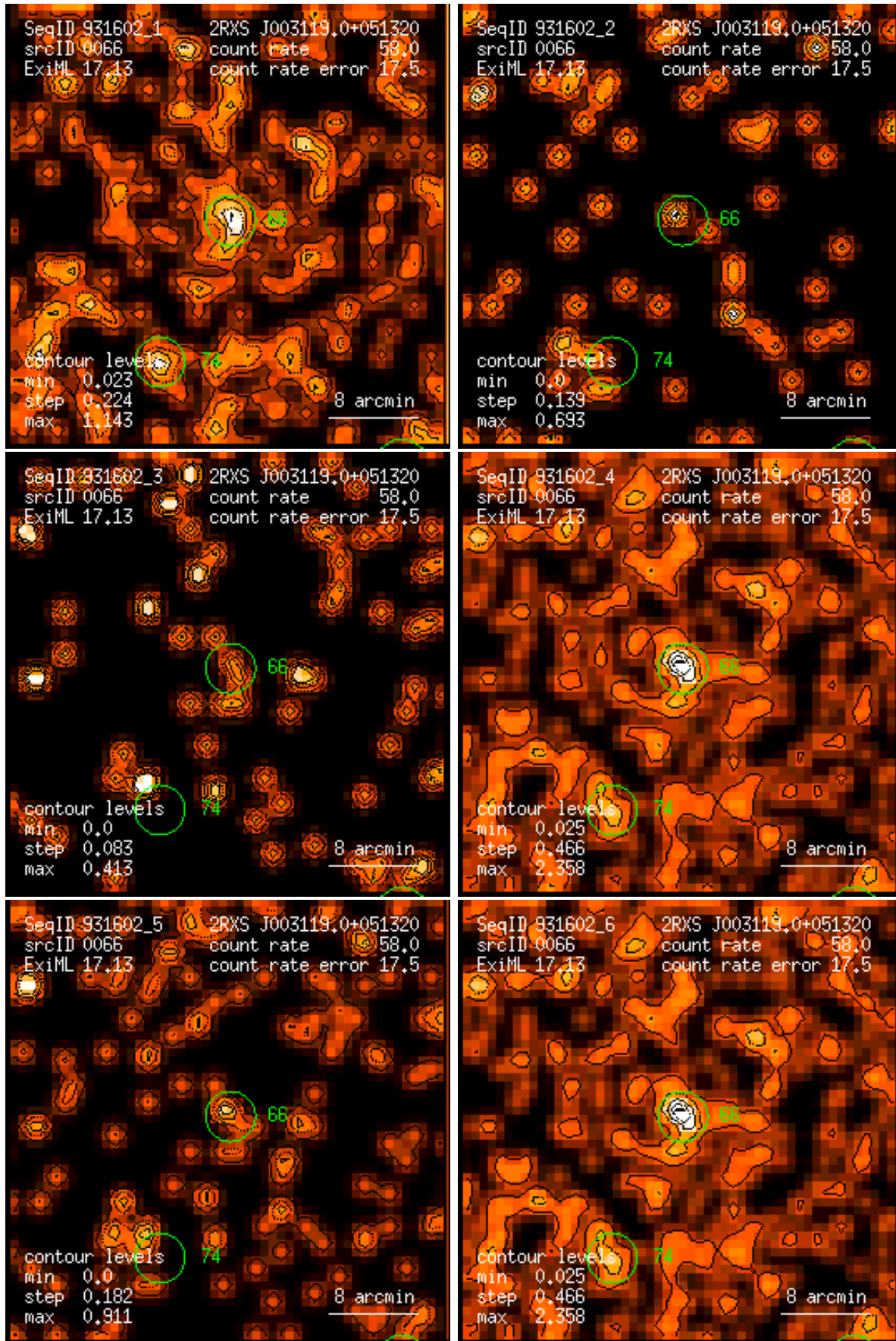
Figure 66: RASS 931602: detection 0066: band rate images, Gaussian filter: (1) PSPC channels 11 – 41, (2) 52 – 90, (3) 91 – 201, (4) 11 – 235, (5) 52 – 201, (6) 11 – 201. Broad band rates in counts/ks. Band rate contour levels in counts/ks/arcmin 2 .
