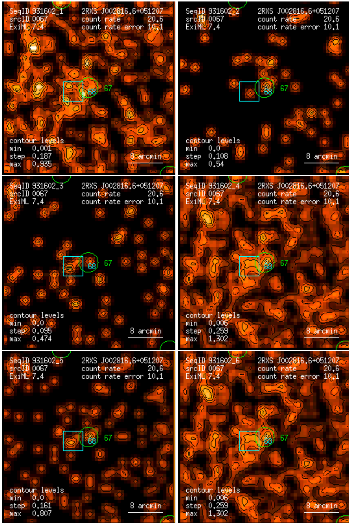
Figure 67: RASS 931602: detection 0067: band rate images, Gaussian filter: (1) PSPC channels 11 – 41, (2) 52 – 90, (3) 91 – 201, (4) 11 – 235, (5) 52 – 201, (6) 11 – 201. Broad band rates in counts/ks. Band rate contour levels in counts/ks/arcmin 2 .
