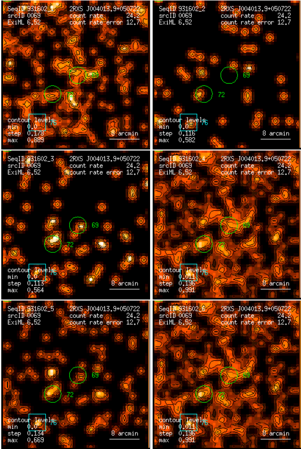
Figure 69: RASS 931602: detection 0069: band rate images, Gaussian filter: (1) PSPC channels 11 – 41, (2) 52 – 90, (3) 91 – 201, (4) 11 – 235, (5) 52 – 201, (6) 11 – 201. Broad band rates in counts/ks. Band rate contour levels in counts/ks/arcmin 2 .
