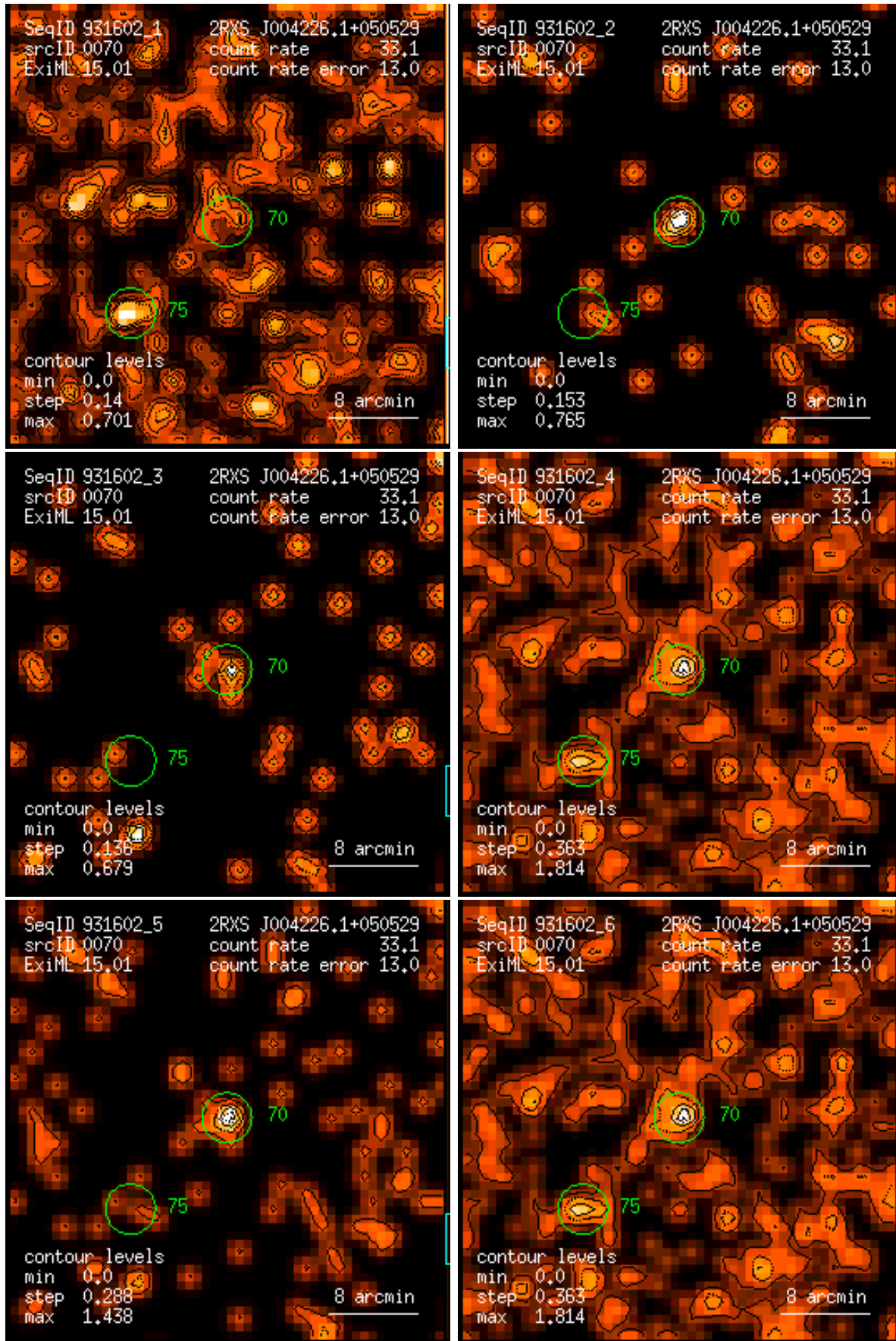
Figure 70: RASS 931602: detection 0070: band rate images, Gaussian filter: (1) PSPC channels 11 – 41, (2) 52 – 90, (3) 91 – 201, (4) 11 – 235, (5) 52 – 201, (6) 11 – 201. Broad band rates in counts/ks. Band rate contour levels in counts/ks/arcmin 2 .
