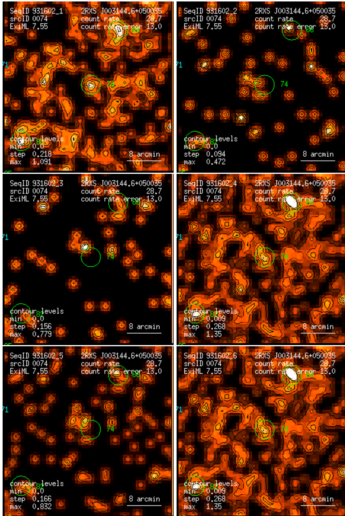
Figure 74: RASS 931602: detection 0074: band rate images, Gaussian filter: (1) PSPC channels 11 – 41, (2) 52 – 90, (3) 91 – 201, (4) 11 – 235, (5) 52 – 201, (6) 11 – 201. Broad band rates in counts/ks. Band rate contour levels in counts/ks/arcmin 2 .
