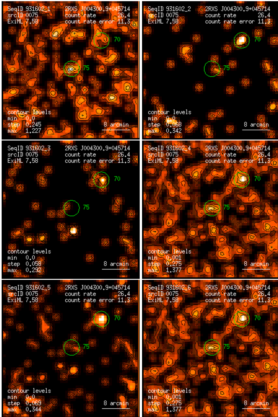
Figure 75: RASS 931602: detection 0075: band rate images, Gaussian filter: (1) PSPC channels 11 – 41, (2) 52 – 90, (3) 91 – 201, (4) 11 – 235, (5) 52 – 201, (6) 11 – 201. Broad band rates in counts/ks. Band rate contour levels in counts/ks/arcmin 2 .
