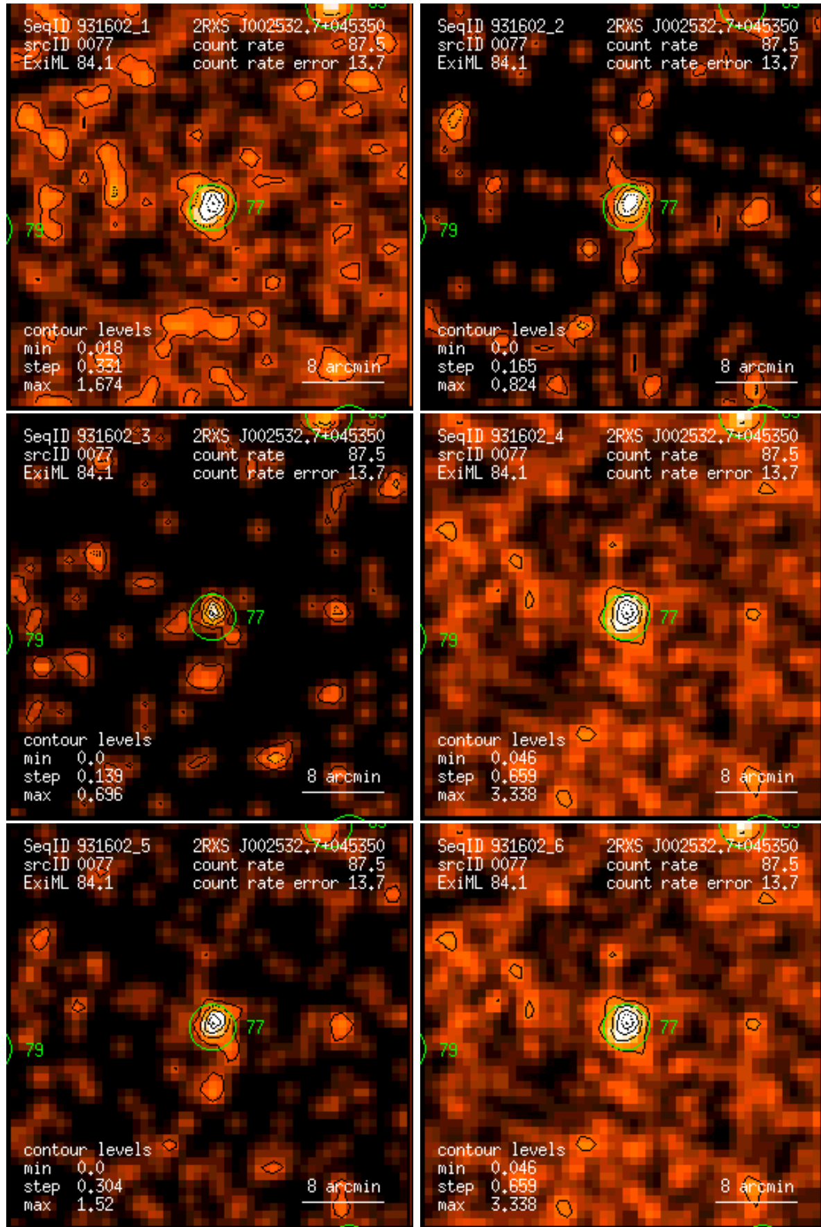
Figure 77: RASS 931602: detection 0077: band rate images, Gaussian filter: (1) PSPC channels 11 – 41, (2) 52 – 90, (3) 91 – 201, (4) 11 – 235, (5) 52 – 201, (6) 11 – 201. Broad band rates in counts/ks. Band rate contour levels in counts/ks/arcmin 2 .
