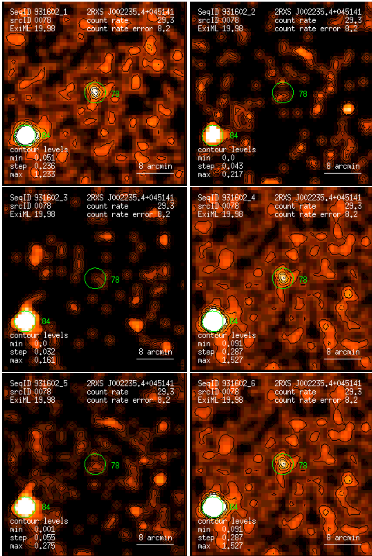
Figure 78: RASS 931602: detection 0078: band rate images, Gaussian filter: (1) PSPC channels 11 – 41, (2) 52 – 90, (3) 91 – 201, (4) 11 – 235, (5) 52 – 201, (6) 11 – 201. Broad band rates in counts/ks. Band rate contour levels in counts/ks/arcmin 2 .
