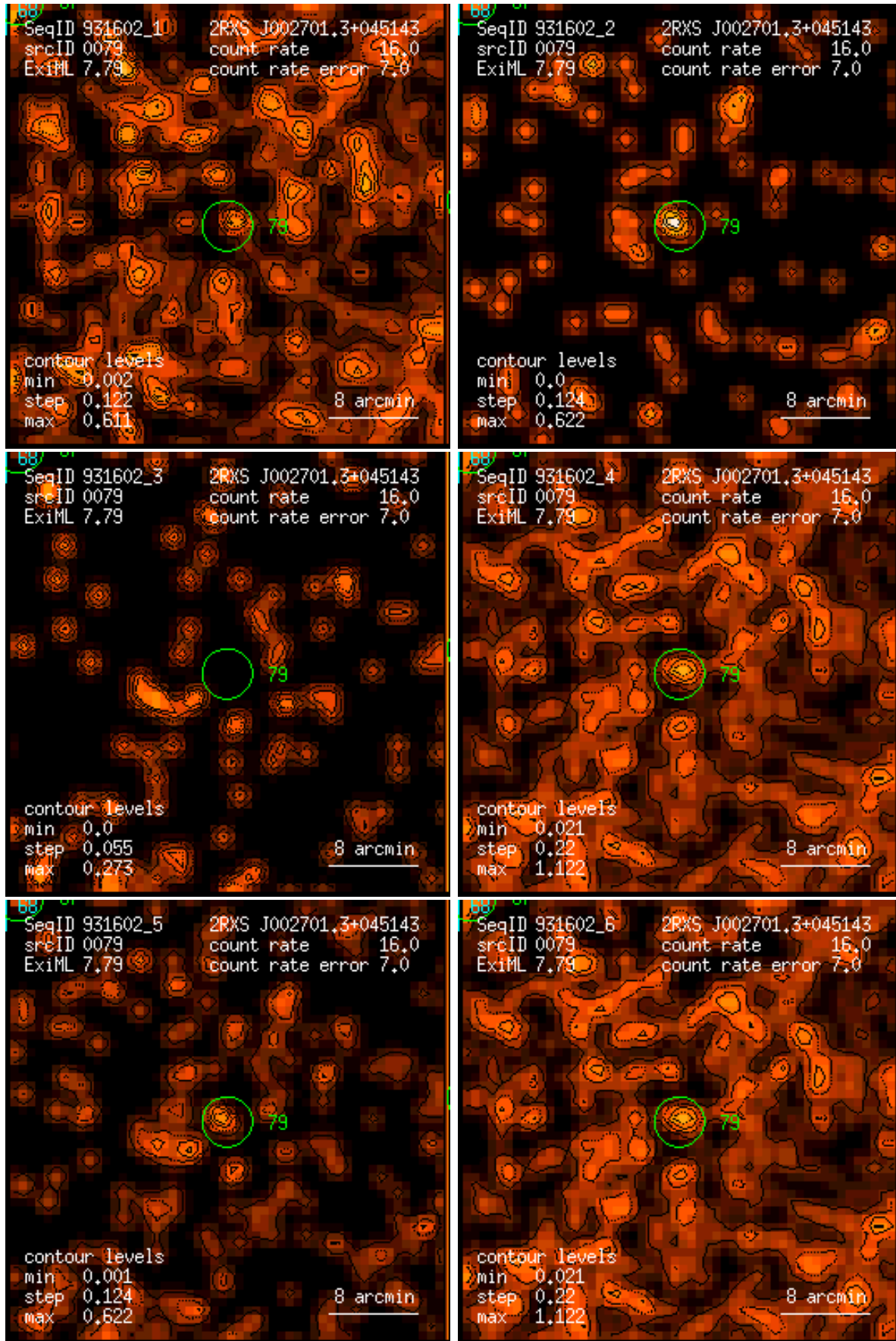
Figure 79: RASS 931602: detection 0079: band rate images, Gaussian filter: (1) PSPC channels 11 – 41, (2) 52 – 90, (3) 91 – 201, (4) 11 – 235, (5) 52 – 201, (6) 11 – 201. Broad band rates in counts/ks. Band rate contour levels in counts/ks/arcmin 2 .
