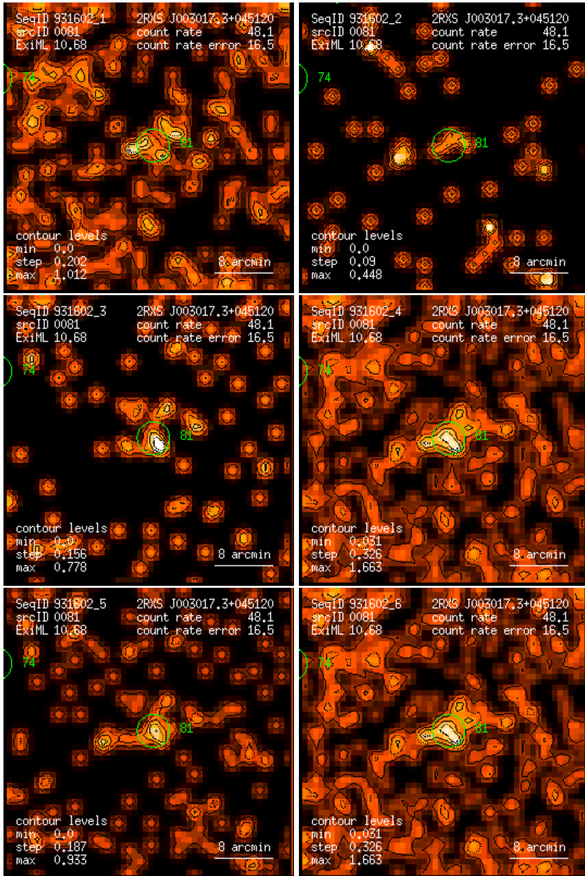
Figure 81: RASS 931602: detection 0081: band rate images, Gaussian filter: (1) PSPC channels 11 – 41, (2) 52 – 90, (3) 91 – 201, (4) 11 – 235, (5) 52 – 201, (6) 11 – 201. Broad band rates in counts/ks. Band rate contour levels in counts/ks/arcmin 2 .
