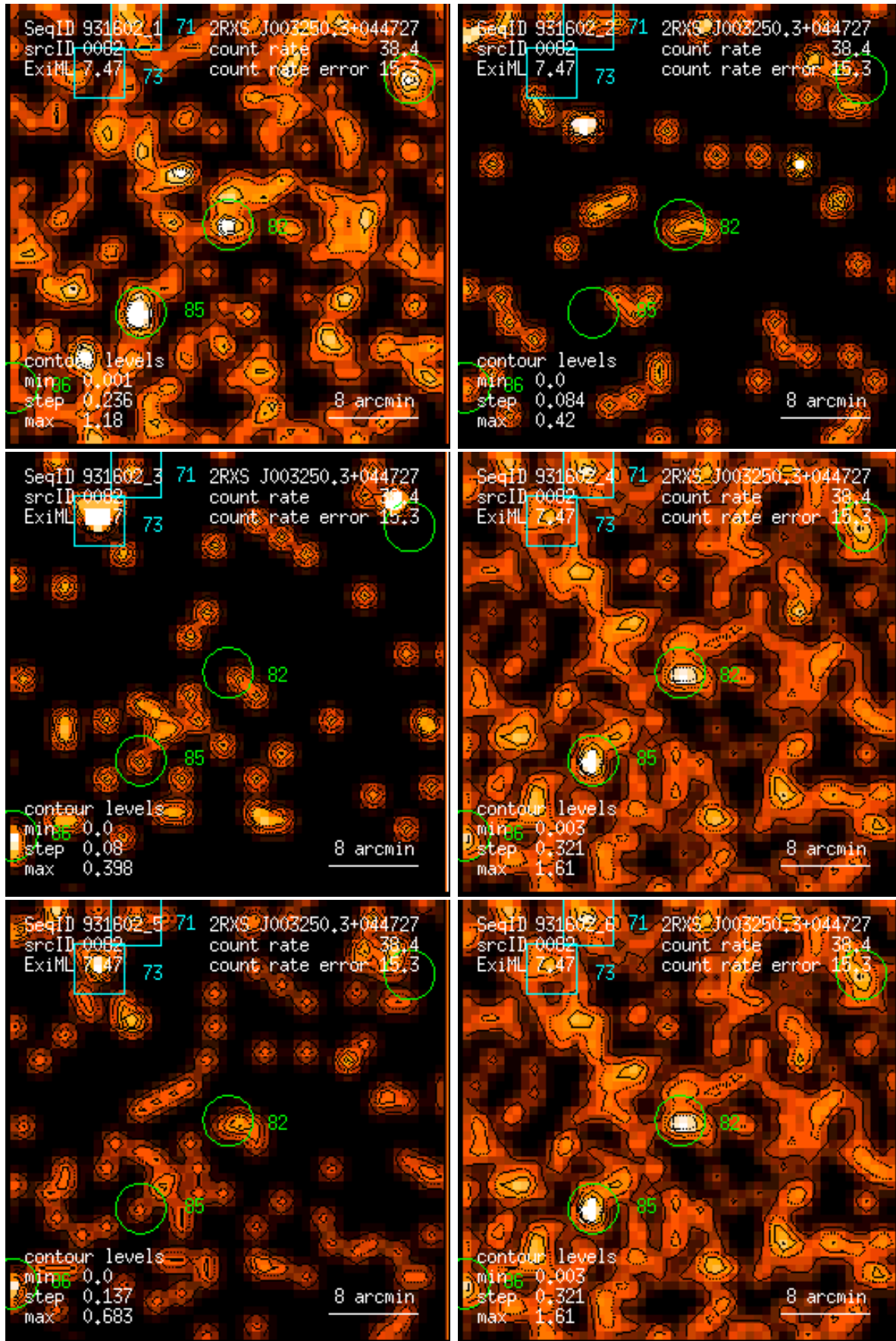
Figure 82: RASS 931602: detection 0082: band rate images, Gaussian filter: (1) PSPC channels 11 – 41, (2) 52 – 90, (3) 91 – 201, (4) 11 – 235, (5) 52 – 201, (6) 11 – 201. Broad band rates in counts/ks. Band rate contour levels in counts/ks/arcmin 2 .
