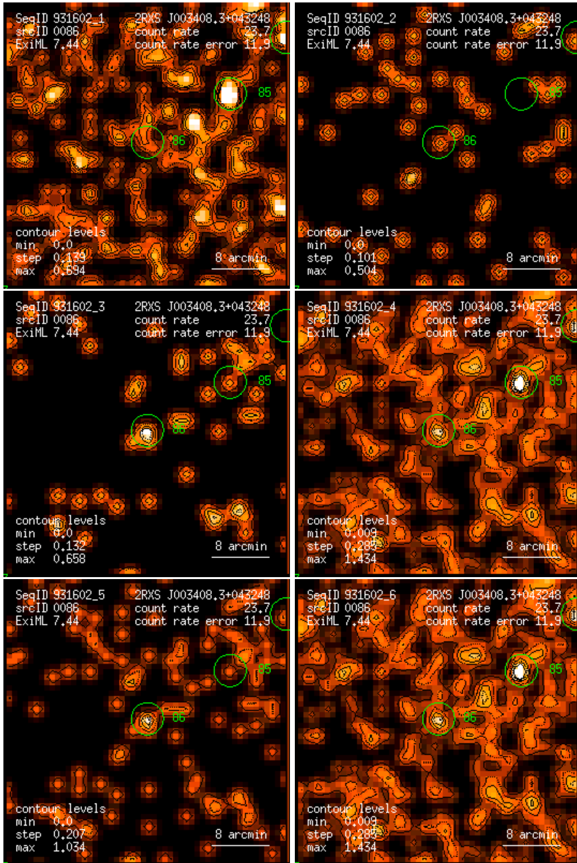
Figure 86: RASS 931602: detection 0086: band rate images, Gaussian filter: (1) PSPC channels 11 – 41, (2) 52 – 90, (3) 91 – 201, (4) 11 – 235, (5) 52 – 201, (6) 11 – 201. Broad band rates in counts/ks. Band rate contour levels in counts/ks/arcmin 2 .
