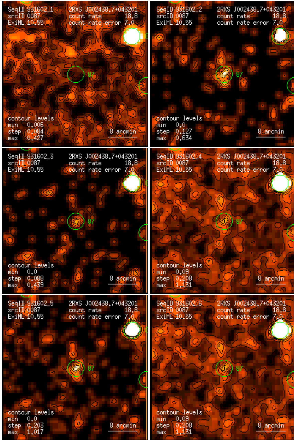
Figure 87: RASS 931602: detection 0087: band rate images, Gaussian filter: (1) PSPC channels 11 – 41, (2) 52 – 90, (3) 91 – 201, (4) 11 – 235, (5) 52 – 201, (6) 11 – 201. Broad band rates in counts/ks. Band rate contour levels in counts/ks/arcmin 2 .
