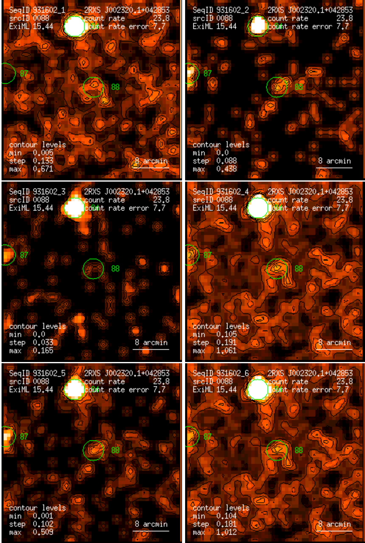
Figure 88: RASS 931602: detection 0088: band rate images, Gaussian filter: (1) PSPC channels 11 – 41, (2) 52 – 90, (3) 91 – 201, (4) 11 – 235, (5) 52 – 201, (6) 11 – 201. Broad band rates in counts/ks. Band rate contour levels in counts/ks/arcmin 2 .
