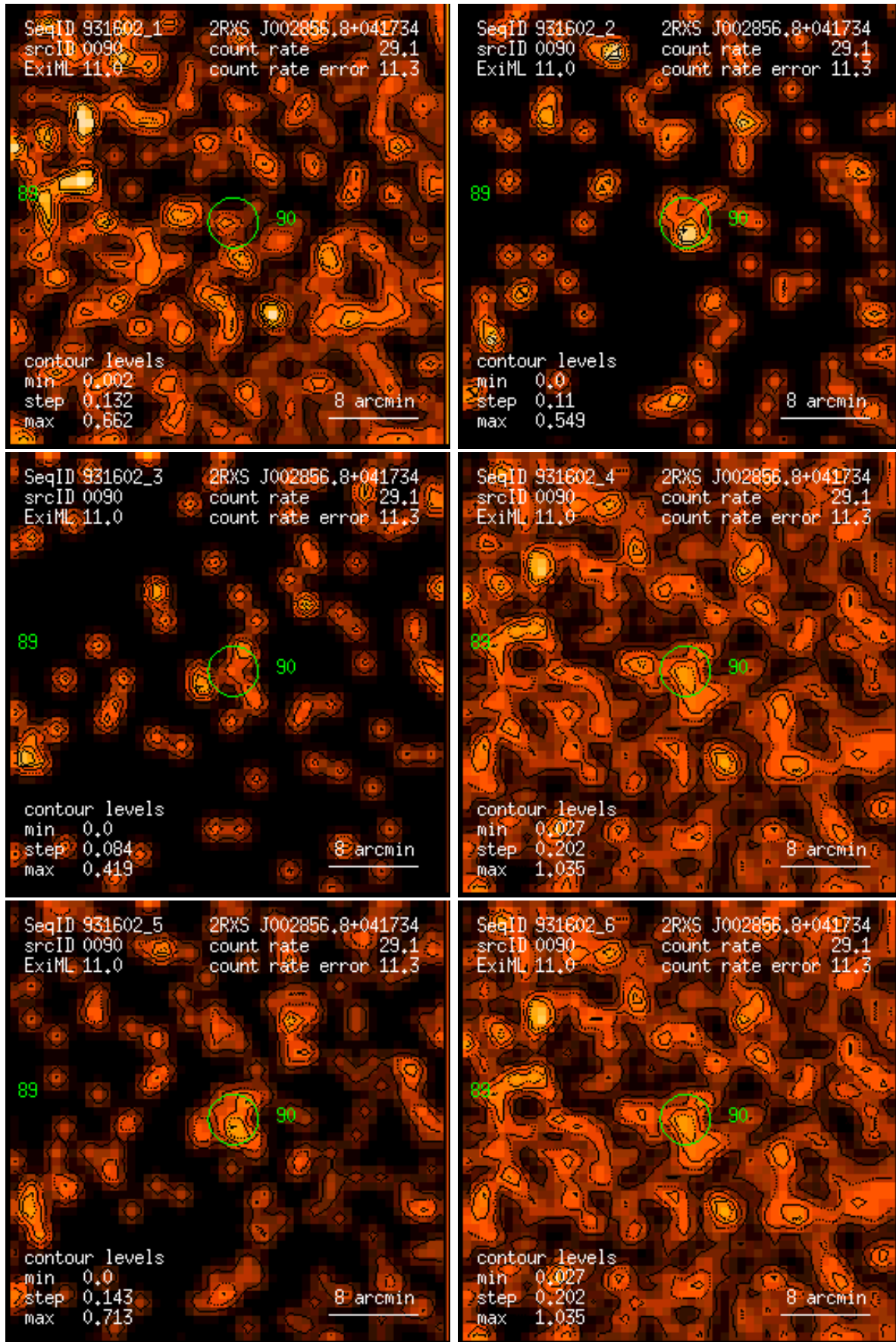
Figure 90: RASS 931602: detection 0090: band rate images, Gaussian filter: (1) PSPC channels 11 – 41, (2) 52 – 90, (3) 91 – 201, (4) 11 – 235, (5) 52 – 201, (6) 11 – 201. Broad band rates in counts/ks. Band rate contour levels in counts/ks/arcmin 2 .
