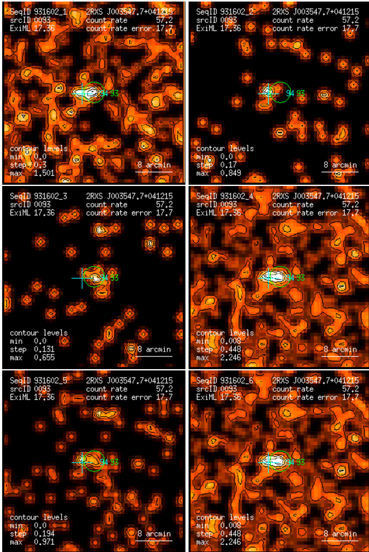
Figure 93: RASS 931602: detection 0093: band rate images, Gaussian filter: (1) PSPC channels 11 – 41, (2) 52 – 90, (3) 91 – 201, (4) 11 – 235, (5) 52 – 201, (6) 11 – 201. Broad band rates in counts/ks. Band rate contour levels in counts/ks/arcmin 2 .
