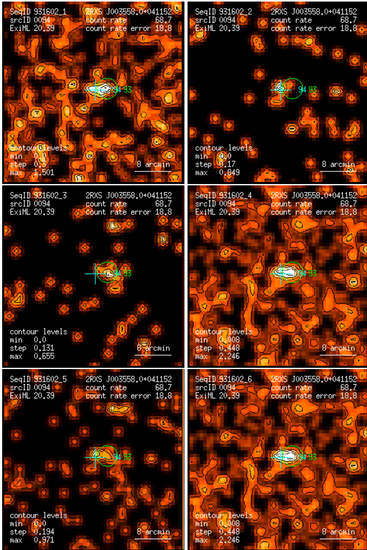
Figure 94: RASS 931602: detection 0094: band rate images, Gaussian filter: (1) PSPC channels 11 – 41, (2) 52 – 90, (3) 91 – 201, (4) 11 – 235, (5) 52 – 201, (6) 11 – 201. Broad band rates in counts/ks. Band rate contour levels in counts/ks/arcmin 2 .
