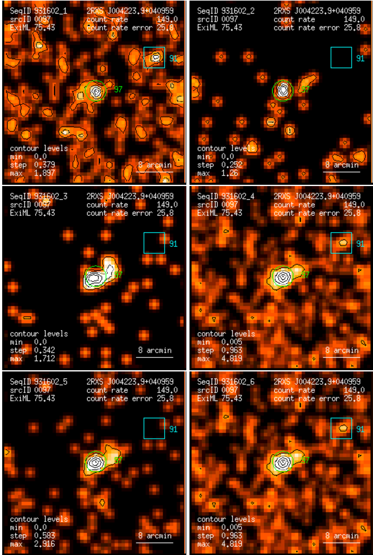
Figure 97: RASS 931602: detection 0097: band rate images, Gaussian filter: (1) PSPC channels 11 – 41, (2) 52 – 90, (3) 91 – 201, (4) 11 – 235, (5) 52 – 201, (6) 11 – 201. Broad band rates in counts/ks. Band rate contour levels in counts/ks/arcmin 2 .
