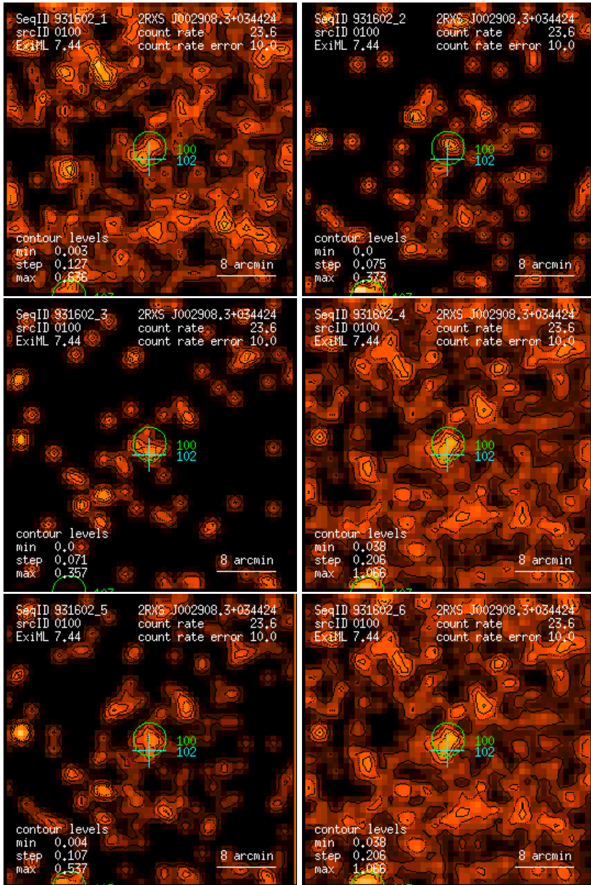
Figure 100: RASS 931602: detection 0100: band rate images, Gaussian filter: (1) PSPC channels 11 – 41, (2) 52 – 90, (3) 91 – 201, (4) 11 – 235, (5) 52 – 201, (6) 11 – 201. Broad band rates in counts/ks. Band rate contour levels in counts/ks/arcmin 2 .
