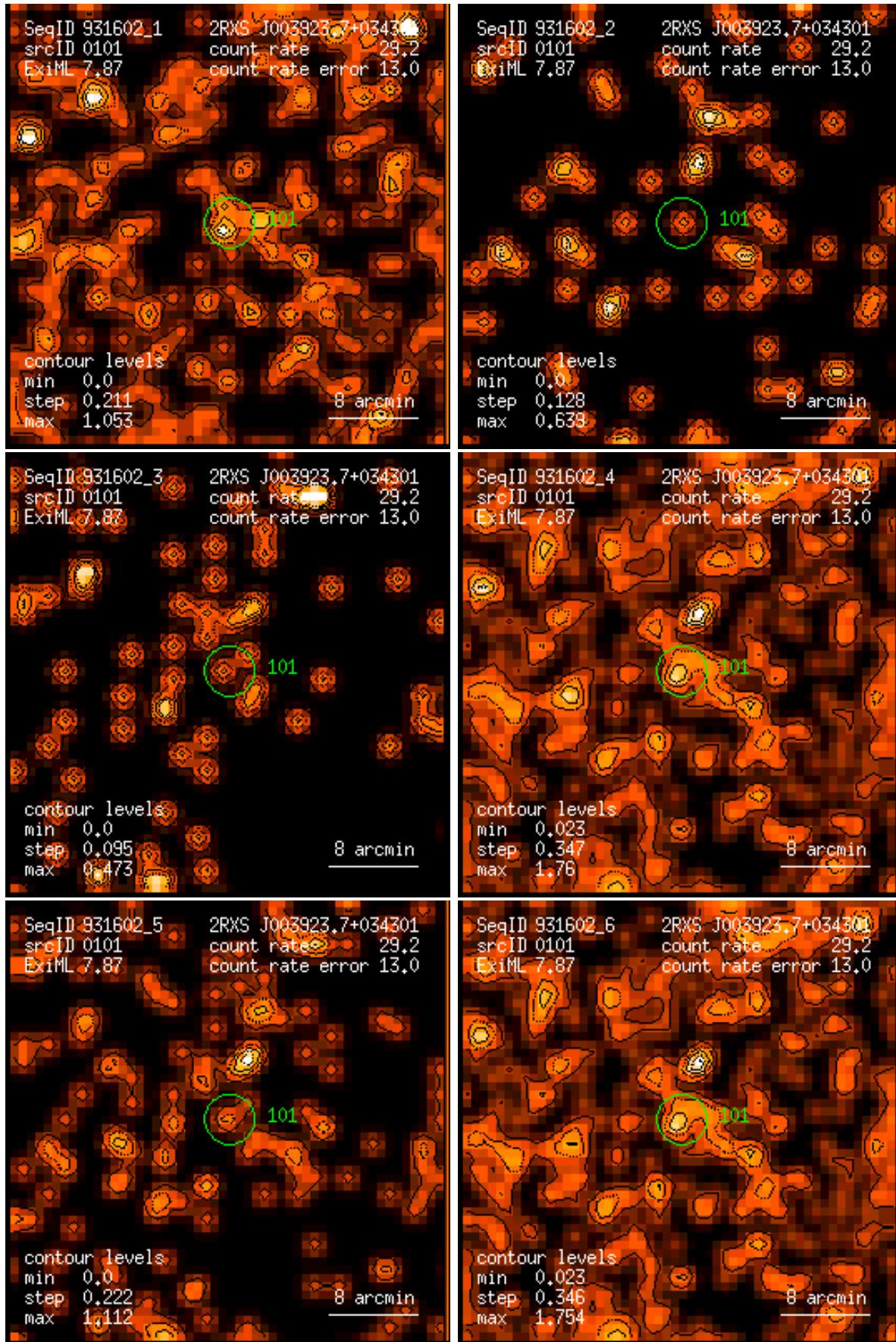
Figure 101: RASS 931602: detection 0101: band rate images, Gaussian filter: (1) PSPC channels 11 – 41, (2) 52 – 90, (3) 91 – 201, (4) 11 – 235, (5) 52 – 201, (6) 11 – 201. Broad band rates in counts/ks. Band rate contour levels in counts/ks/arcmin 2 .
