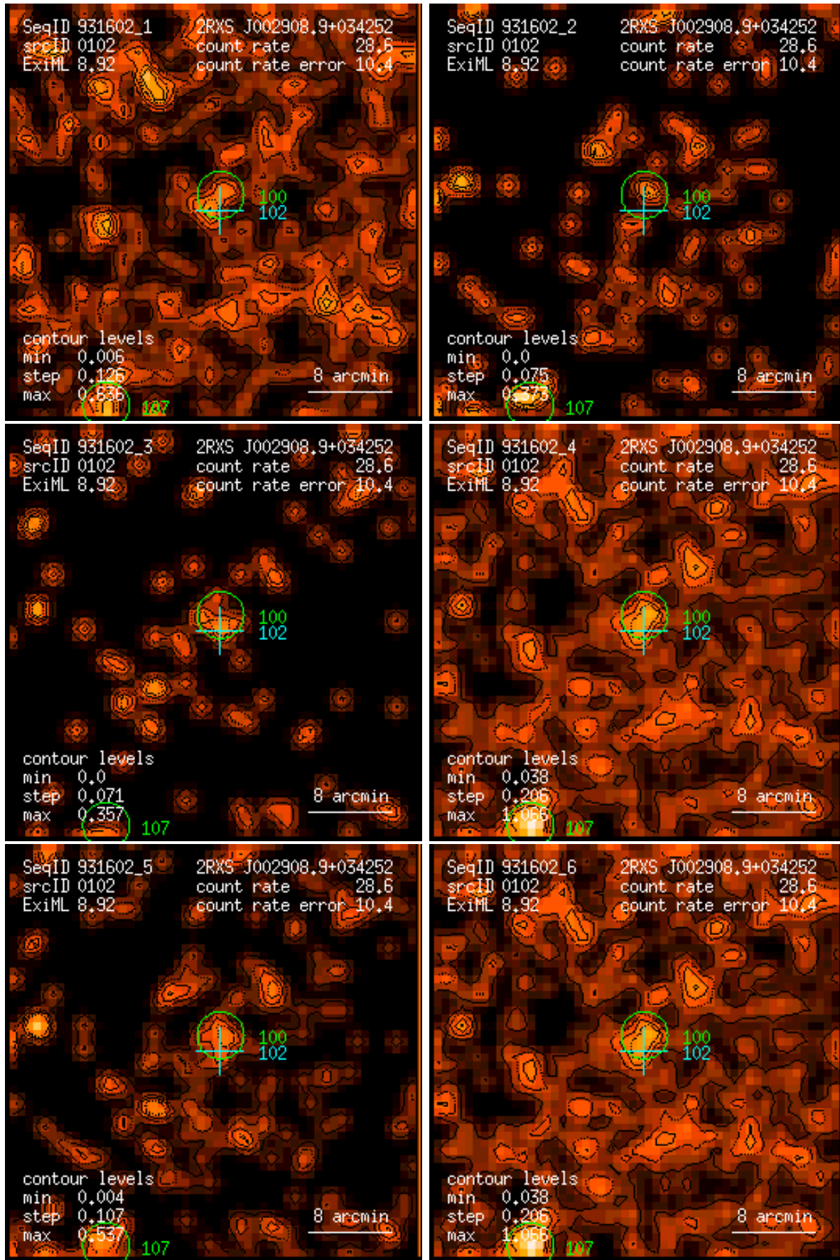
Figure 102: RASS 931602: detection 0102: band rate images, Gaussian filter: (1) PSPC channels 11 – 41, (2) 52 – 90, (3) 91 – 201, (4) 11 – 235, (5) 52 – 201, (6) 11 – 201. Broad band rates in counts/ks. Band rate contour levels in counts/ks/arcmin 2 .
