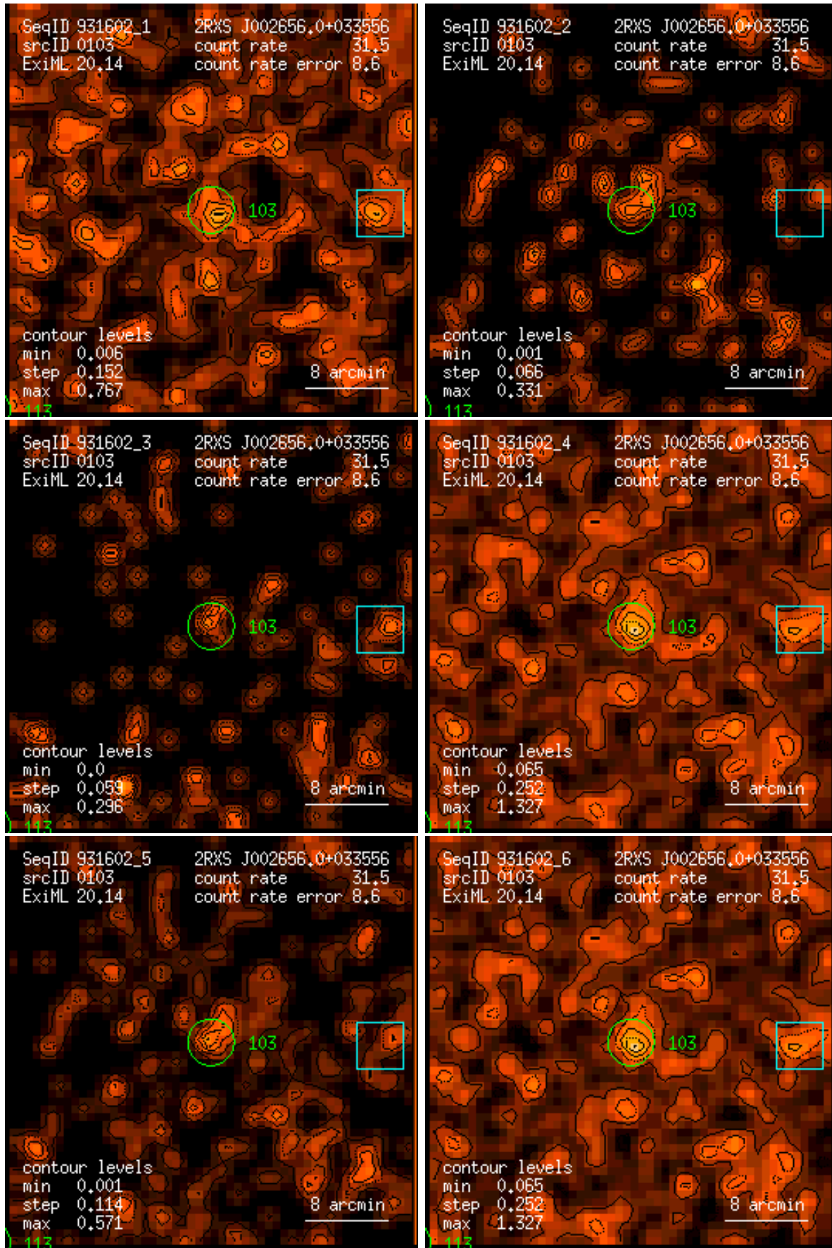
Figure 103: RASS 931602: detection 0103: band rate images, Gaussian filter: (1) PSPC channels 11 – 41, (2) 52 – 90, (3) 91 – 201, (4) 11 – 235, (5) 52 – 201, (6) 11 – 201. Broad band rates in counts/ks. Band rate contour levels in counts/ks/arcmin 2 .
