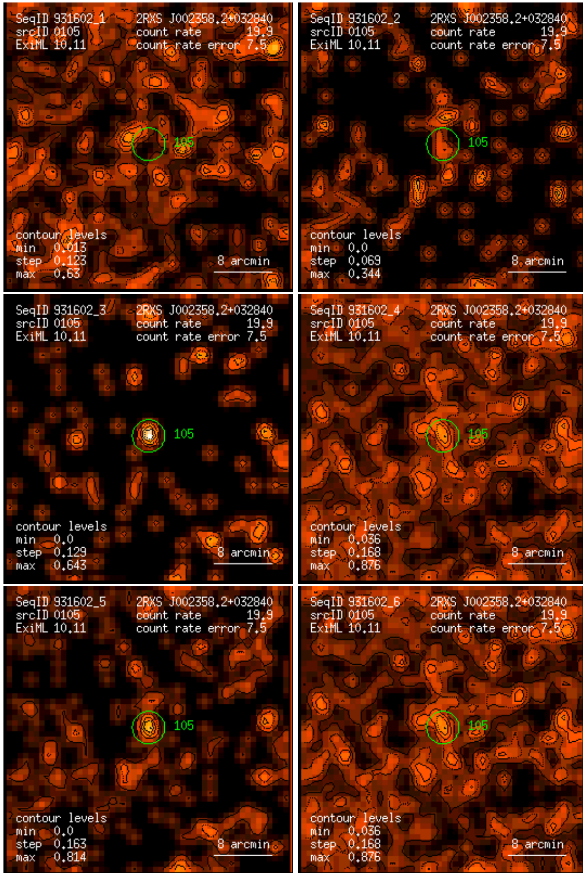
Figure 105: RASS 931602: detection 0105: band rate images, Gaussian filter: (1) PSPC channels 11 – 41, (2) 52 – 90, (3) 91 – 201, (4) 11 – 235, (5) 52 – 201, (6) 11 – 201. Broad band rates in counts/ks. Band rate contour levels in counts/ks/arcmin 2 .
