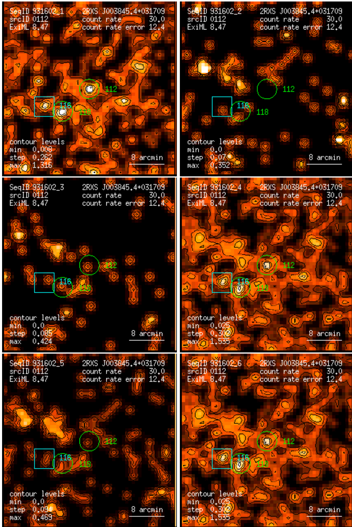
Figure 112: RASS 931602: detection 0112: band rate images, Gaussian filter: (1) PSPC channels 11 – 41, (2) 52 – 90, (3) 91 – 201, (4) 11 – 235, (5) 52 – 201, (6) 11 – 201. Broad band rates in counts/ks. Band rate contour levels in counts/ks/arcmin 2 .
