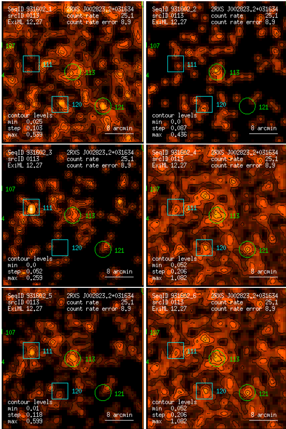
Figure 113: RASS 931602: detection 0113: band rate images, Gaussian filter: (1) PSPC channels 11 – 41, (2) 52 – 90, (3) 91 – 201, (4) 11 – 235, (5) 52 – 201, (6) 11 – 201. Broad band rates in counts/ks. Band rate contour levels in counts/ks/arcmin 2 .
