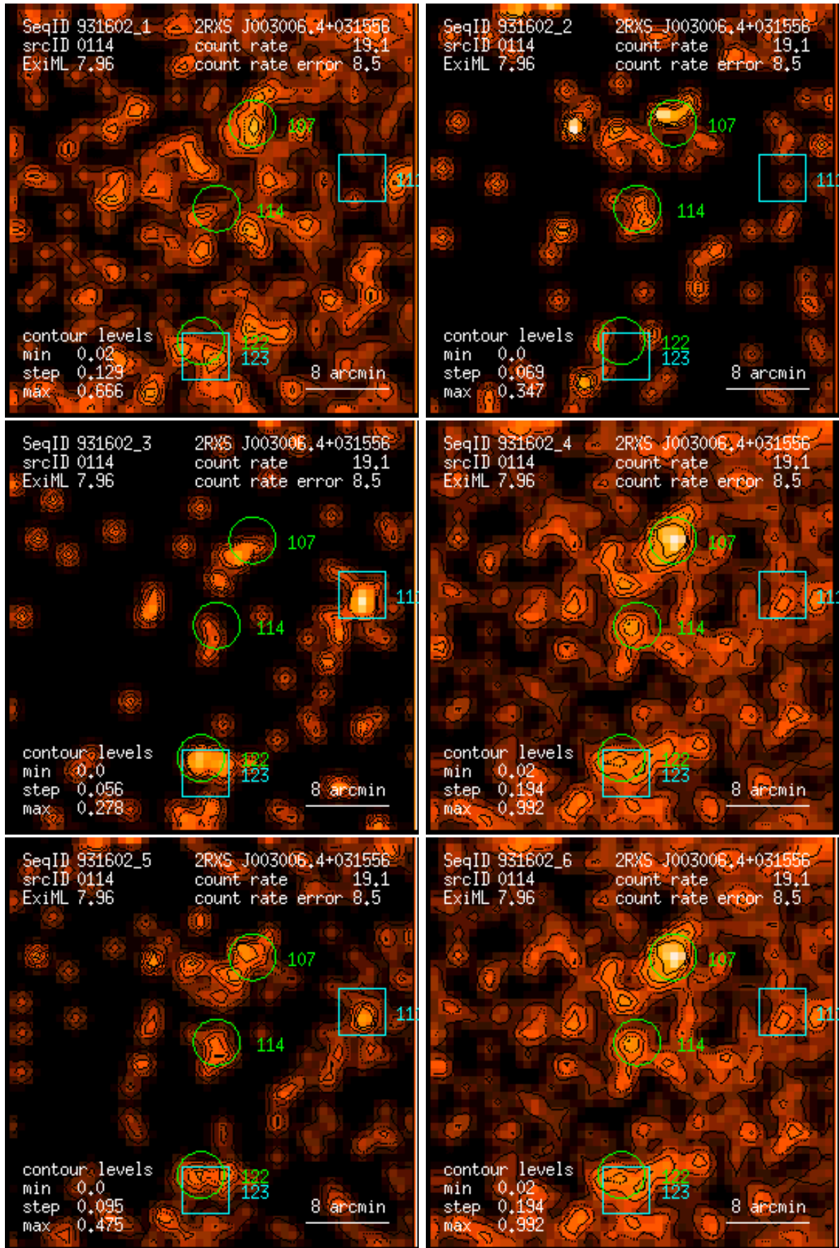
Figure 114: RASS 931602: detection 0114: band rate images, Gaussian filter: (1) PSPC channels 11 – 41, (2) 52 – 90, (3) 91 – 201, (4) 11 – 235, (5) 52 – 201, (6) 11 – 201. Broad band rates in counts/ks. Band rate contour levels in counts/ks/arcmin 2 .
