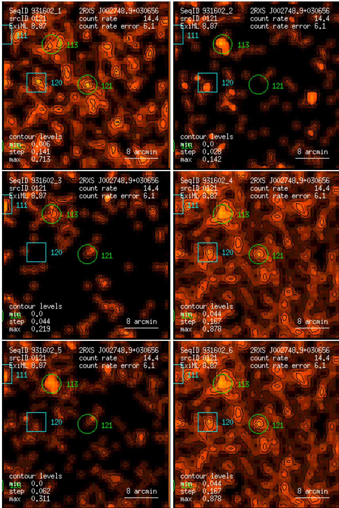
Figure 121: RASS 931602: detection 0121: band rate images, Gaussian filter: (1) PSPC channels 11 – 41, (2) 52 – 90, (3) 91 – 201, (4) 11 – 235, (5) 52 – 201, (6) 11 – 201. Broad band rates in counts/ks. Band rate contour levels in counts/ks/arcmin 2 .
