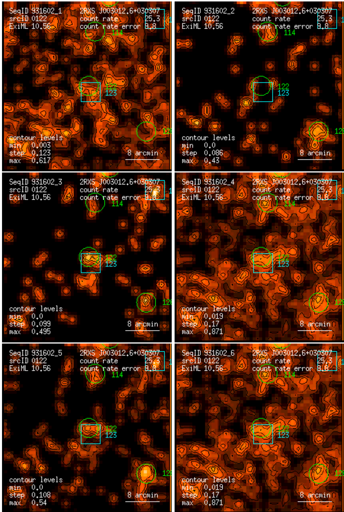
Figure 122: RASS 931602: detection 0122: band rate images, Gaussian filter: (1) PSPC channels 11 – 41, (2) 52 – 90, (3) 91 – 201, (4) 11 – 235, (5) 52 – 201, (6) 11 – 201. Broad band rates in counts/ks. Band rate contour levels in counts/ks/arcmin 2 .
