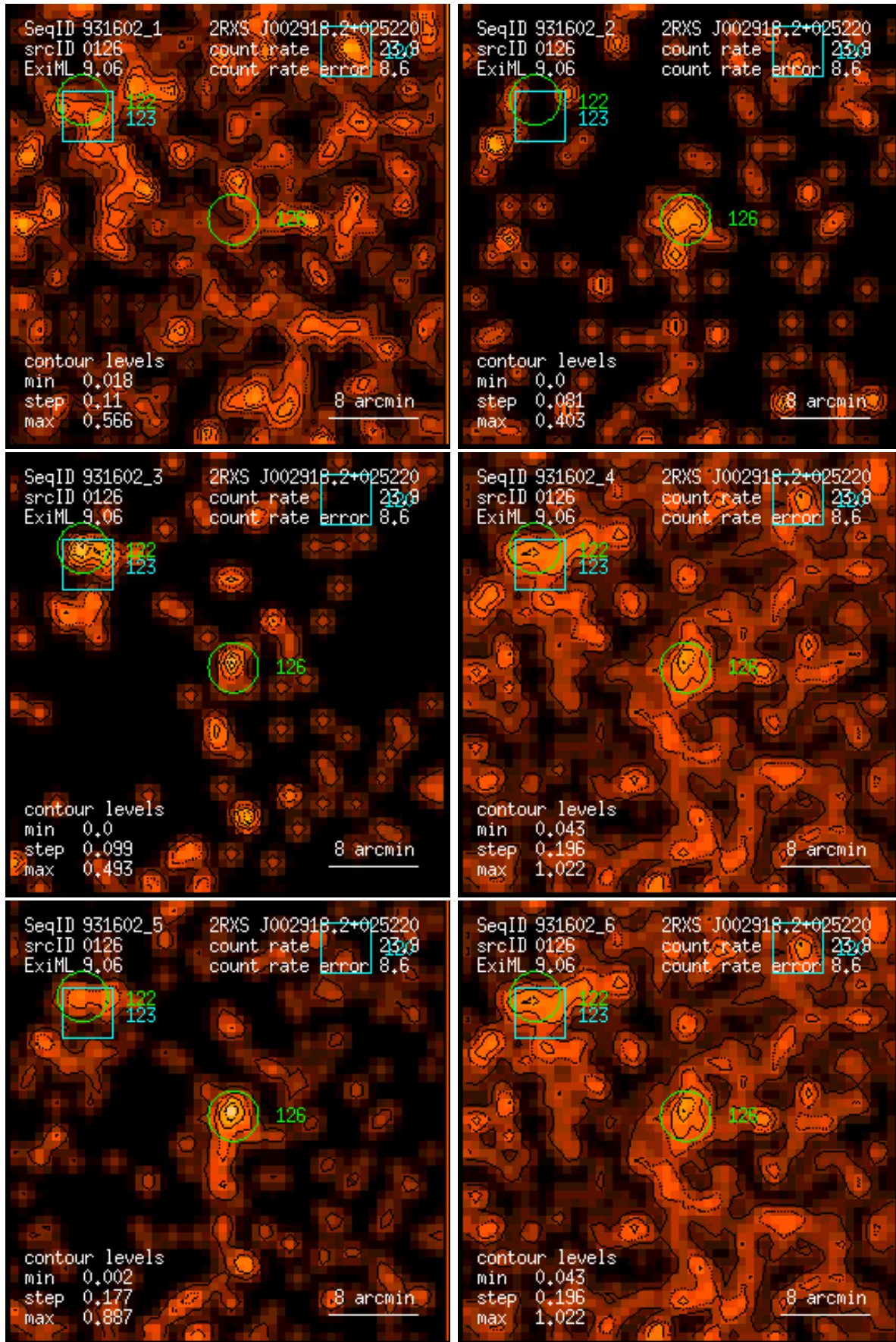
Figure 126: RASS 931602: detection 0126: band rate images, Gaussian filter: (1) PSPC channels 11 – 41, (2) 52 – 90, (3) 91 – 201, (4) 11 – 235, (5) 52 – 201, (6) 11 – 201. Broad band rates in counts/ks. Band rate contour levels in counts/ks/arcmin 2 .
