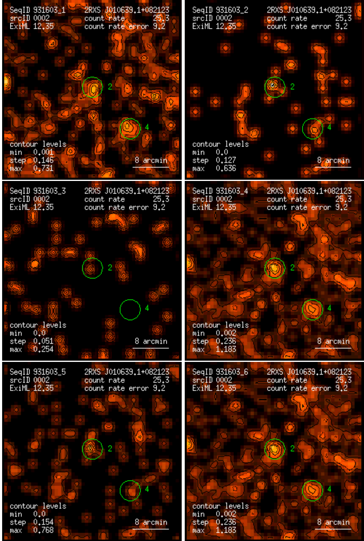
Figure 2: RASS 931603: detection 0002: band rate images, Gaussian filter: (1) PSPC channels 11 – 41, (2) 52 – 90, (3) 91 – 201, (4) 11 – 235, (5) 52 – 201, (6) 11 – 201. Broad band rates in counts/ks. Band rate contour levels in counts/ks/arcmin 2 .
