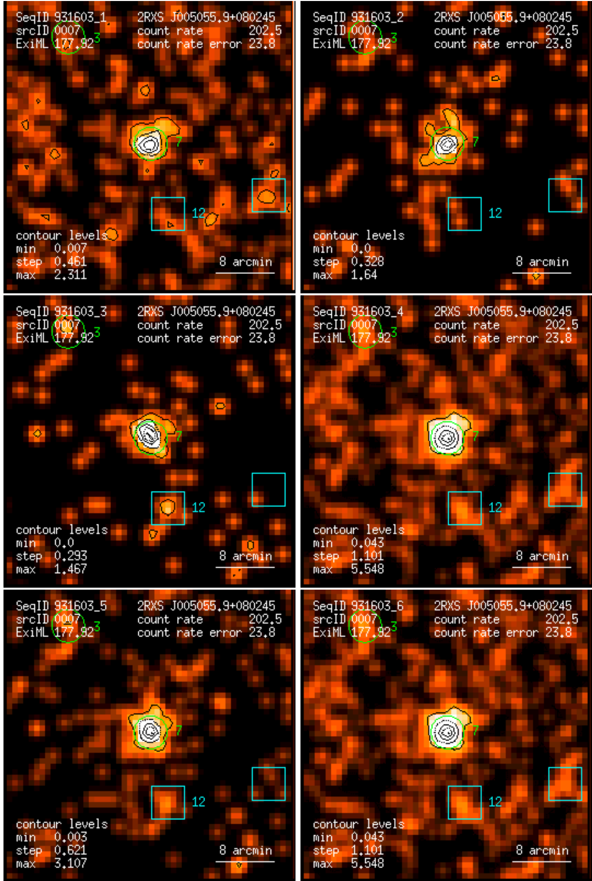
Figure 7: RASS 931603: detection 0007: band rate images, Gaussian filter: (1) PSPC channels 11 – 41, (2) 52 – 90, (3) 91 – 201, (4) 11 – 235, (5) 52 – 201, (6) 11 – 201. Broad band rates in counts/ks. Band rate contour levels in counts/ks/arcmin 2 .
