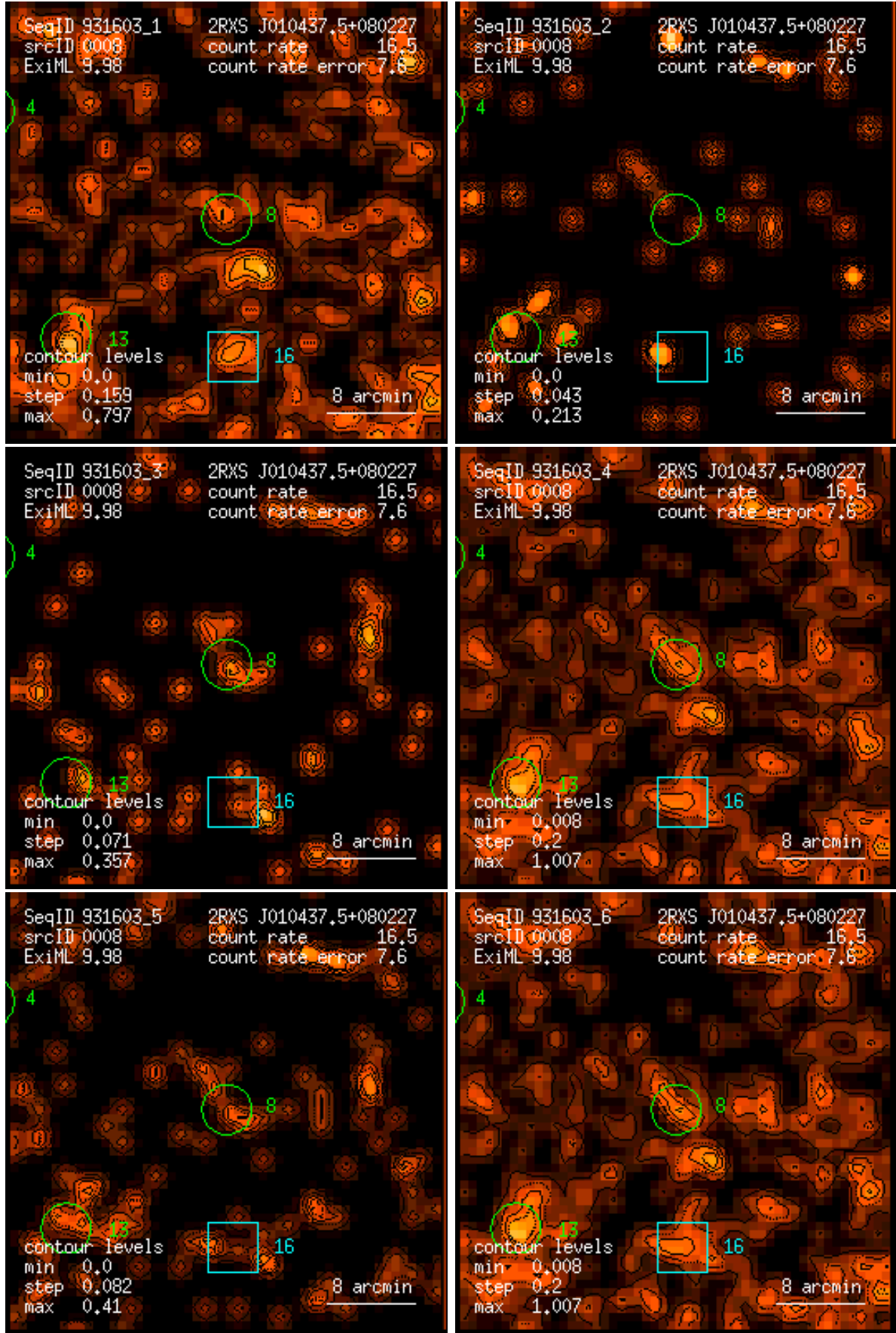
Figure 8: RASS 931603: detection 0008: band rate images, Gaussian filter: (1) PSPC channels 11 – 41, (2) 52 – 90, (3) 91 – 201, (4) 11 – 235, (5) 52 – 201, (6) 11 – 201. Broad band rates in counts/ks. Band rate contour levels in counts/ks/arcmin 2 .
