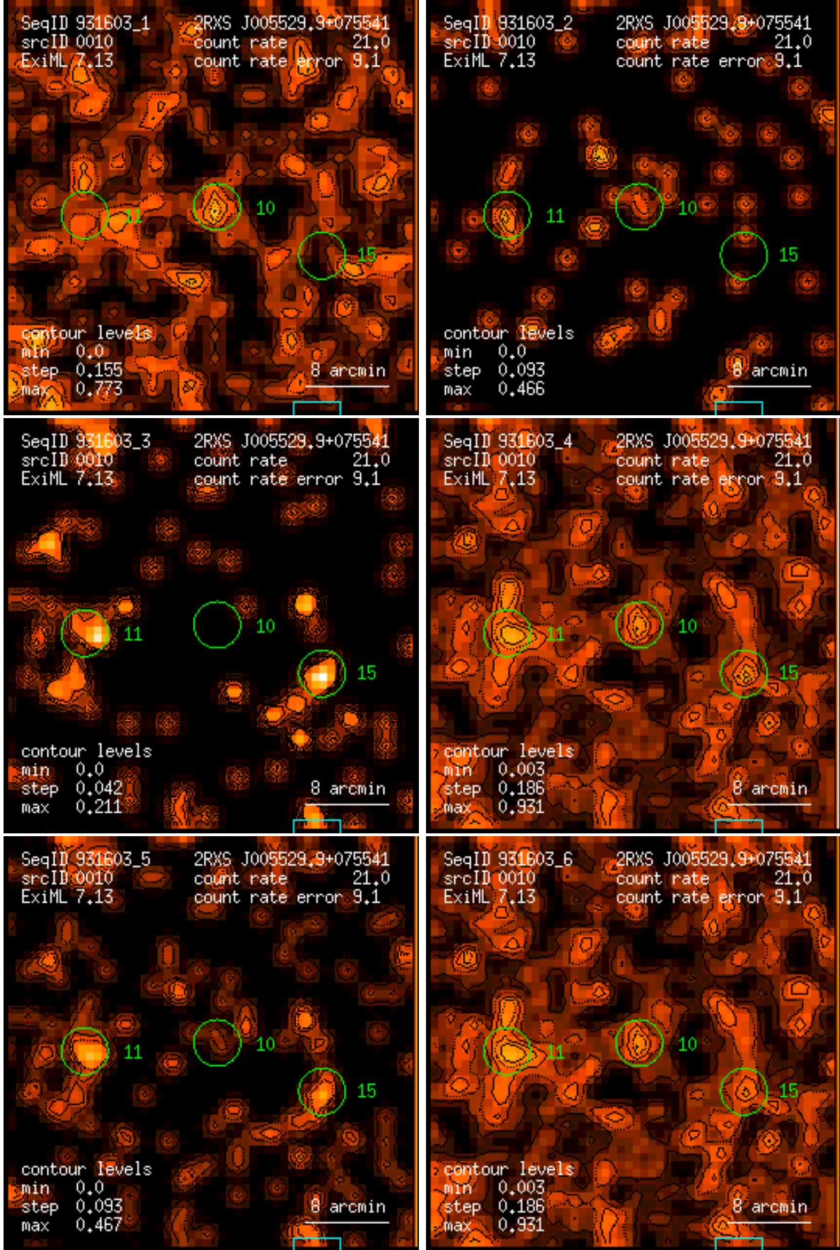
Figure 10: RASS 931603: detection 0010: band rate images, Gaussian filter: (1) PSPC channels 11 – 41, (2) 52 – 90, (3) 91 – 201, (4) 11 – 235, (5) 52 – 201, (6) 11 – 201. Broad band rates in counts/ks. Band rate contour levels in counts/ks/arcmin 2 .
