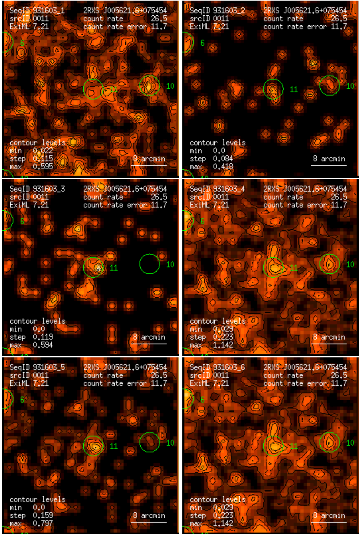
Figure 11: RASS 931603: detection 0011: band rate images, Gaussian filter: (1) PSPC channels 11 – 41, (2) 52 – 90, (3) 91 – 201, (4) 11 – 235, (5) 52 – 201, (6) 11 – 201. Broad band rates in counts/ks. Band rate contour levels in counts/ks/arcmin 2 .
