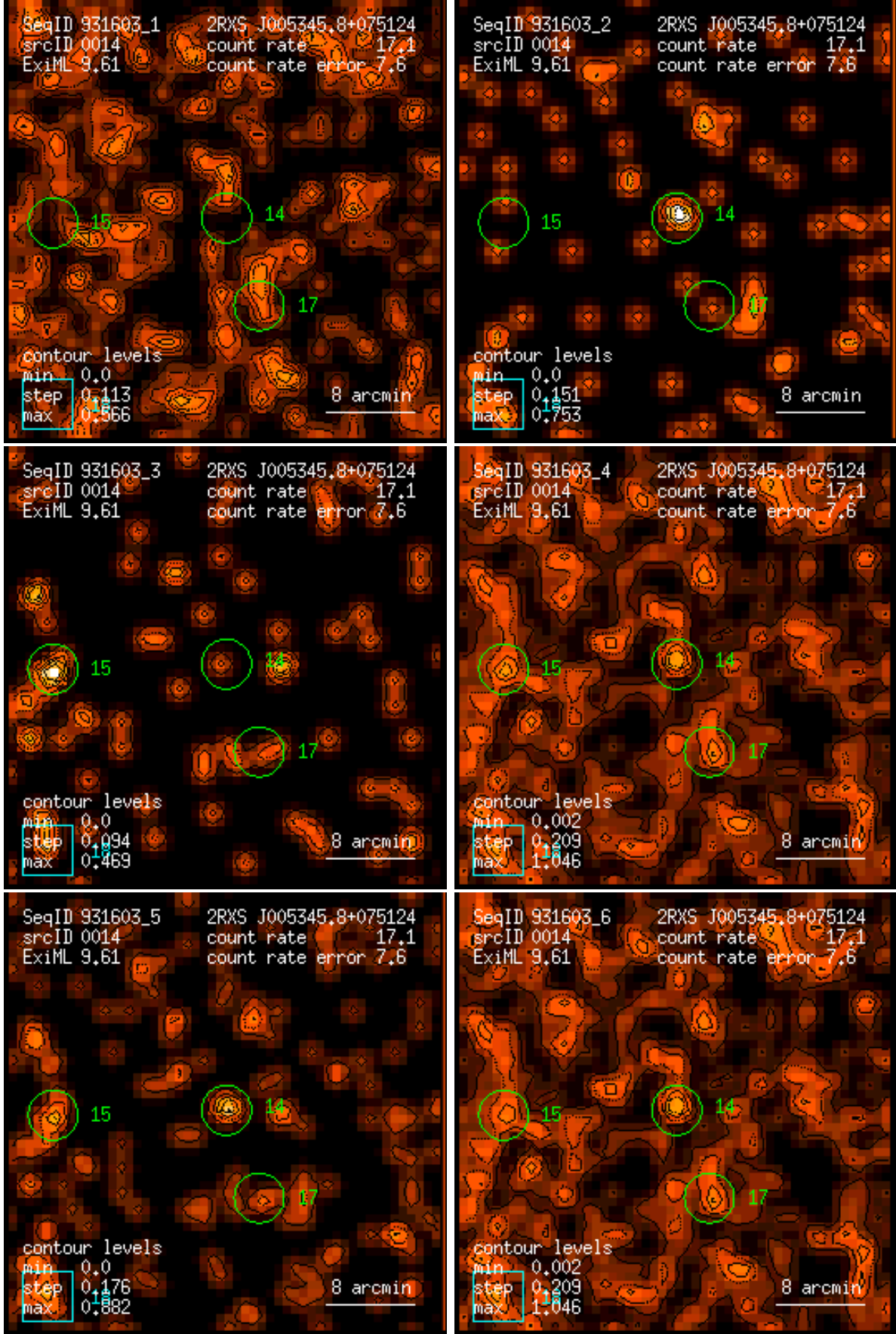
Figure 14: RASS 931603: detection 0014: band rate images, Gaussian filter: (1) PSPC channels 11 – 41, (2) 52 – 90, (3) 91 – 201, (4) 11 – 235, (5) 52 – 201, (6) 11 – 201. Broad band rates in counts/ks. Band rate contour levels in counts/ks/arcmin 2 .
