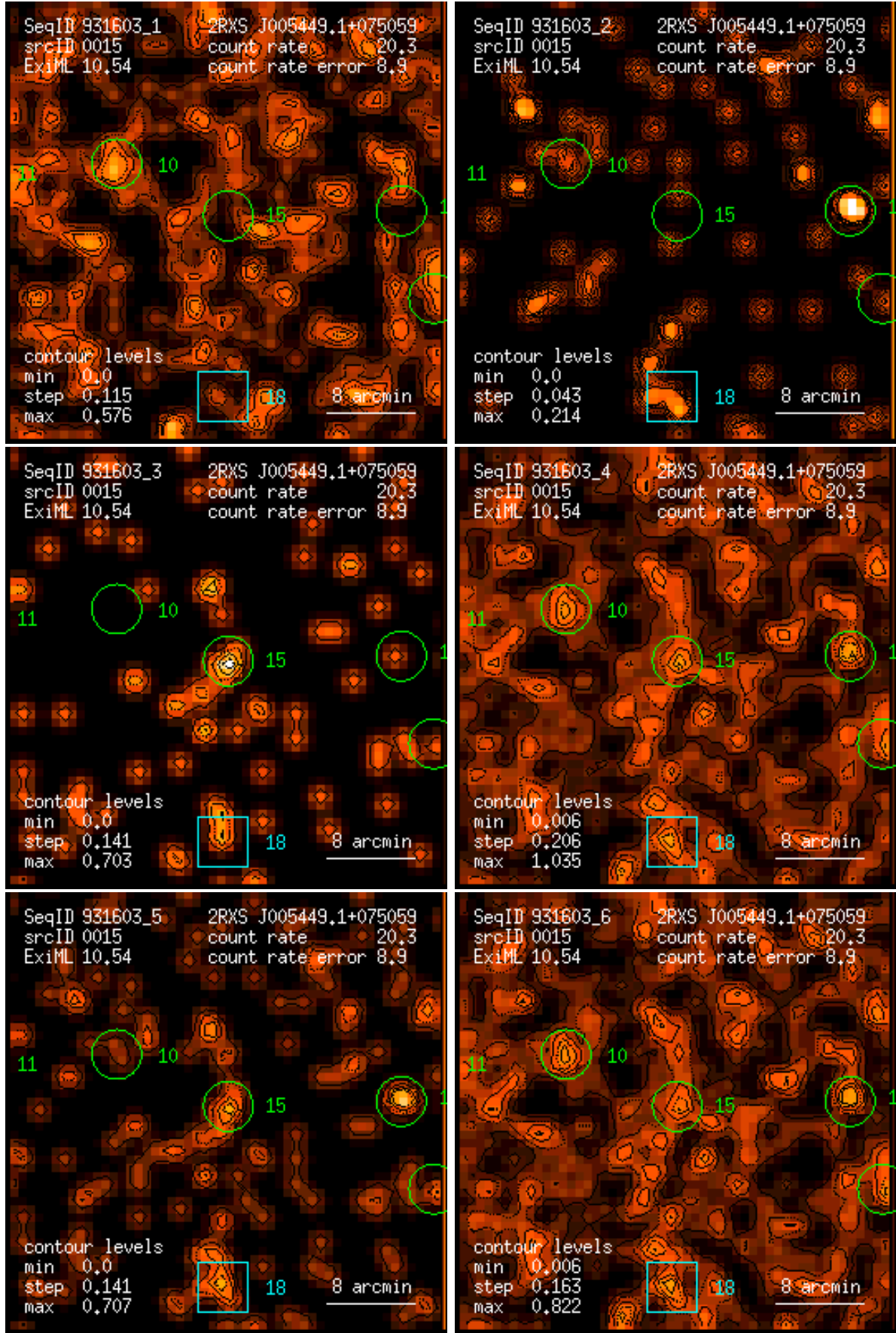
Figure 15: RASS 931603: detection 0015: band rate images, Gaussian filter: (1) PSPC channels 11 – 41, (2) 52 – 90, (3) 91 – 201, (4) 11 – 235, (5) 52 – 201, (6) 11 – 201. Broad band rates in counts/ks. Band rate contour levels in counts/ks/arcmin 2 .
