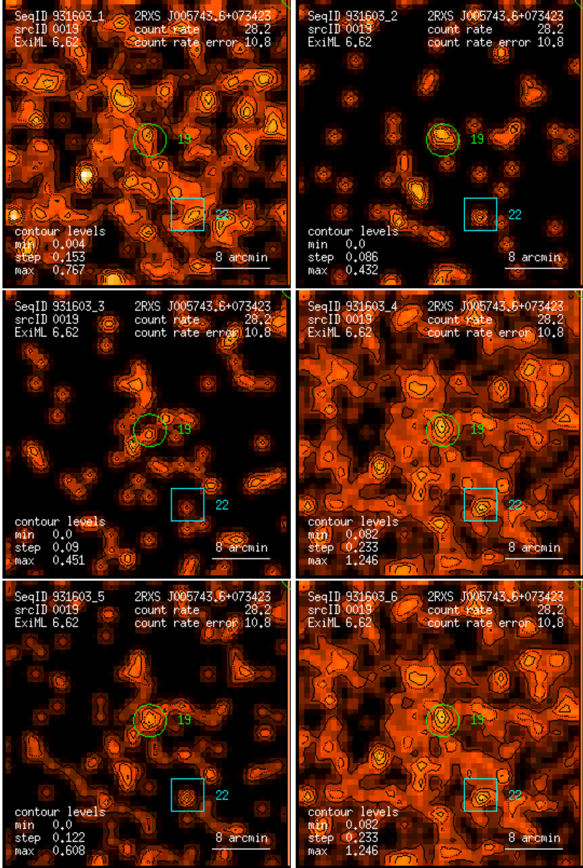
Figure 19: RASS 931603: detection 0019: band rate images, Gaussian filter: (1) PSPC channels 11 – 41, (2) 52 – 90, (3) 91 – 201, (4) 11 – 235, (5) 52 – 201, (6) 11 – 201. Broad band rates in counts/ks. Band rate contour levels in counts/ks/arcmin 2 .
