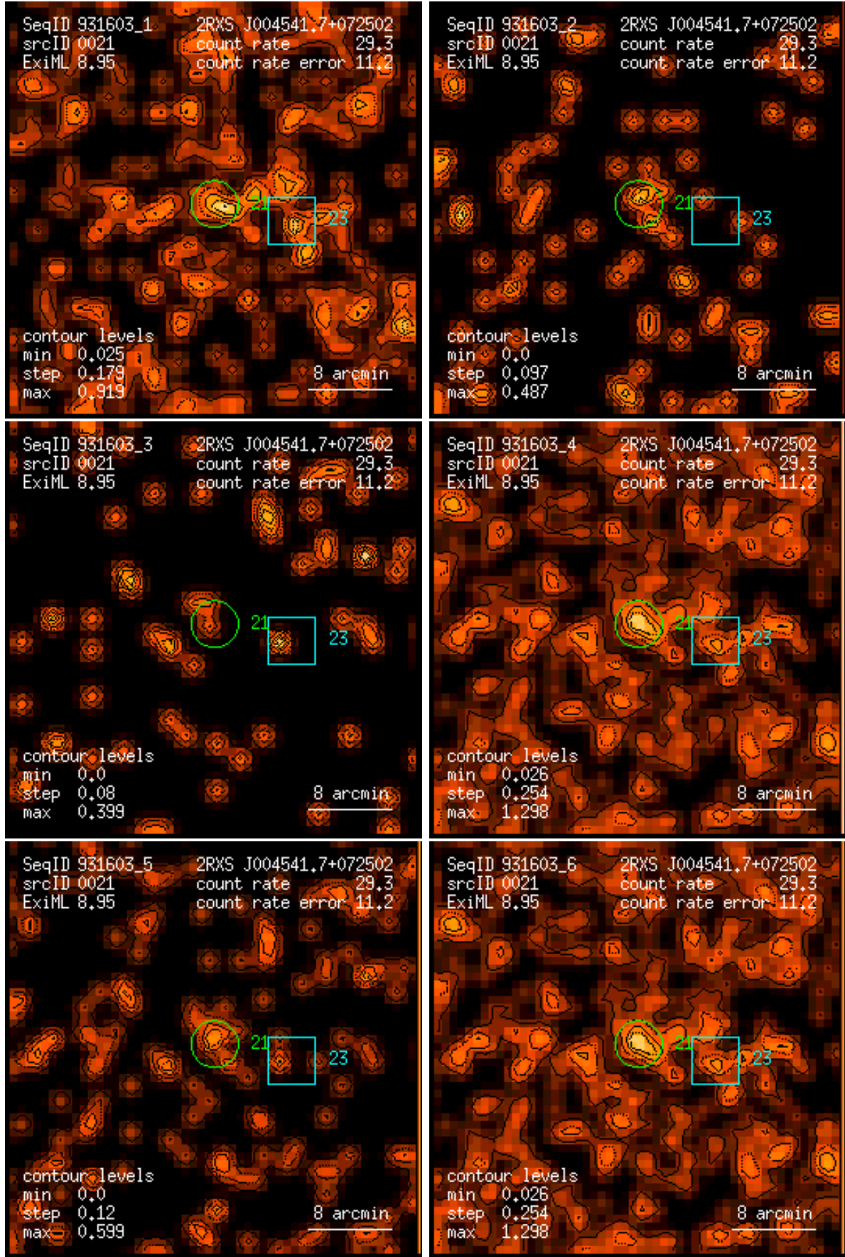
Figure 21: RASS 931603: detection 0021: band rate images, Gaussian filter: (1) PSPC channels 11 – 41, (2) 52 – 90, (3) 91 – 201, (4) 11 – 235, (5) 52 – 201, (6) 11 – 201. Broad band rates in counts/ks. Band rate contour levels in counts/ks/arcmin 2 .
