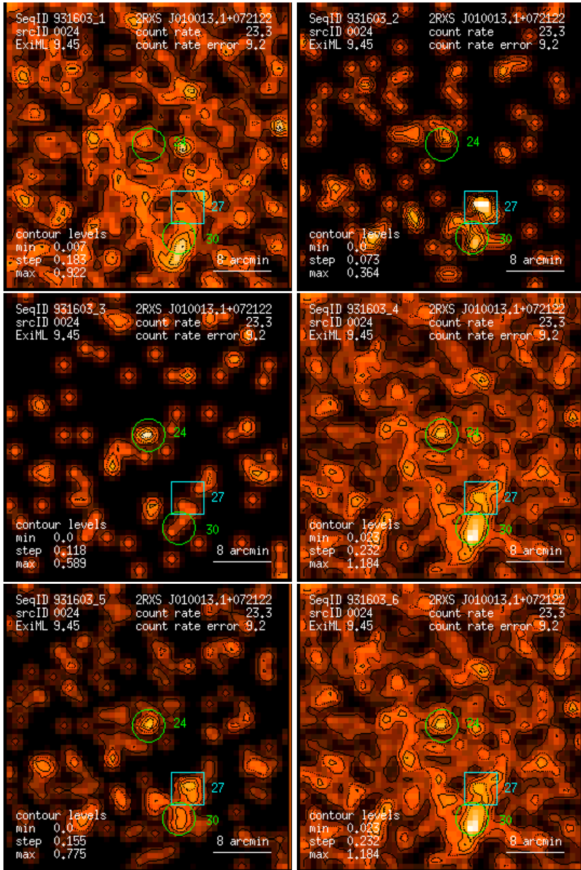
Figure 24: RASS 931603: detection 0024: band rate images, Gaussian filter: (1) PSPC channels 11 – 41, (2) 52 – 90, (3) 91 – 201, (4) 11 – 235, (5) 52 – 201, (6) 11 – 201. Broad band rates in counts/ks. Band rate contour levels in counts/ks/arcmin 2 .
