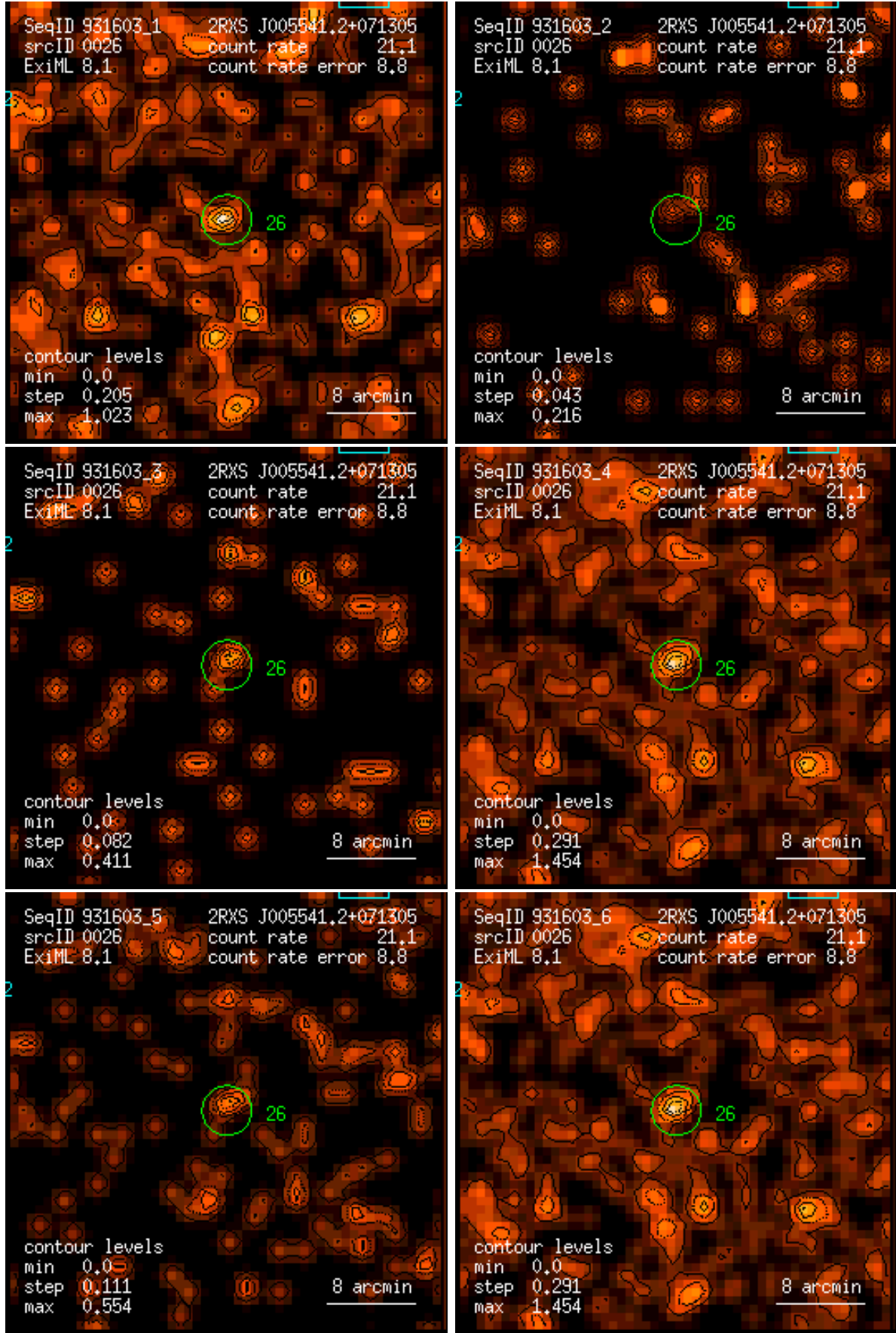
Figure 26: RASS 931603: detection 0026: band rate images, Gaussian filter: (1) PSPC channels 11 – 41, (2) 52 – 90, (3) 91 – 201, (4) 11 – 235, (5) 52 – 201, (6) 11 – 201. Broad band rates in counts/ks. Band rate contour levels in counts/ks/arcmin 2 .
