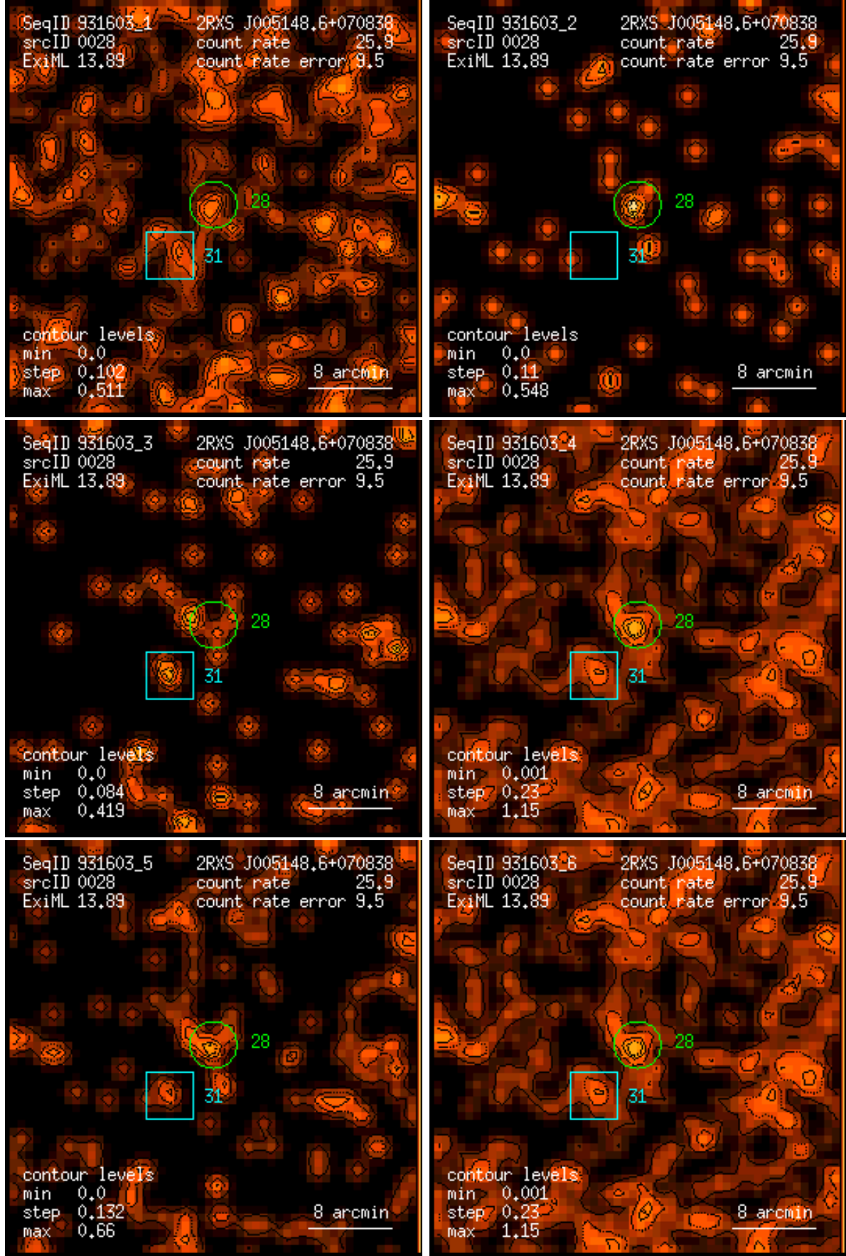
Figure 28: RASS 931603: detection 0028: band rate images, Gaussian filter: (1) PSPC channels 11 – 41, (2) 52 – 90, (3) 91 – 201, (4) 11 – 235, (5) 52 – 201, (6) 11 – 201. Broad band rates in counts/ks. Band rate contour levels in counts/ks/arcmin 2 .
