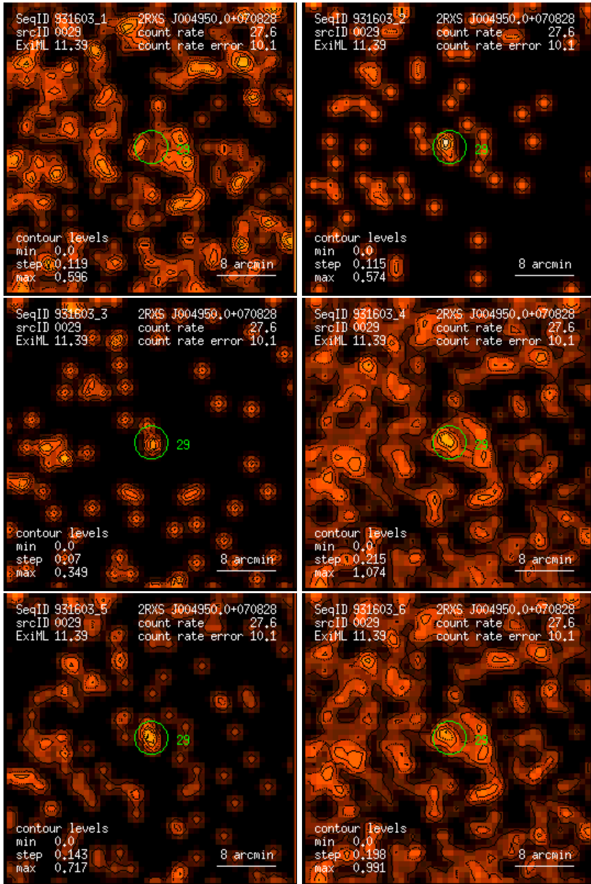
Figure 29: RASS 931603: detection 0029: band rate images, Gaussian filter: (1) PSPC channels 11 – 41, (2) 52 – 90, (3) 91 – 201, (4) 11 – 235, (5) 52 – 201, (6) 11 – 201. Broad band rates in counts/ks. Band rate contour levels in counts/ks/arcmin 2 .
