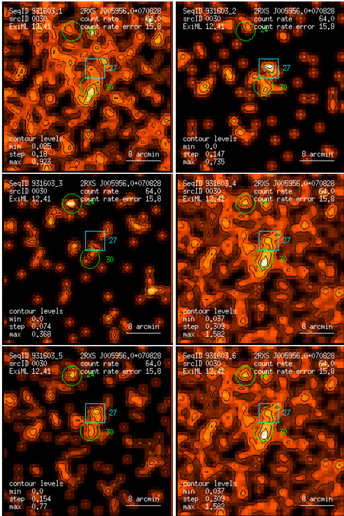
Figure 30: RASS 931603: detection 0030: band rate images, Gaussian filter: (1) PSPC channels 11 – 41, (2) 52 – 90, (3) 91 – 201, (4) 11 – 235, (5) 52 – 201, (6) 11 – 201. Broad band rates in counts/ks. Band rate contour levels in counts/ks/arcmin 2 .
