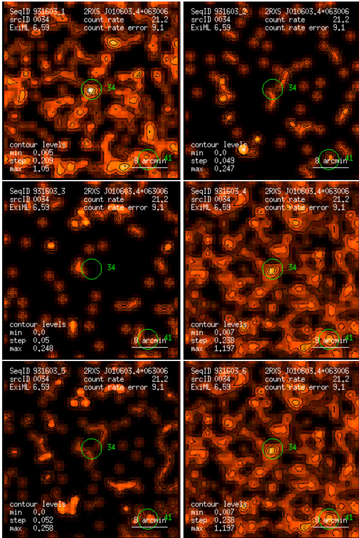
Figure 34: RASS 931603: detection 0034: band rate images, Gaussian filter: (1) PSPC channels 11 – 41, (2) 52 – 90, (3) 91 – 201, (4) 11 – 235, (5) 52 – 201, (6) 11 – 201. Broad band rates in counts/ks. Band rate contour levels in counts/ks/arcmin 2 .
