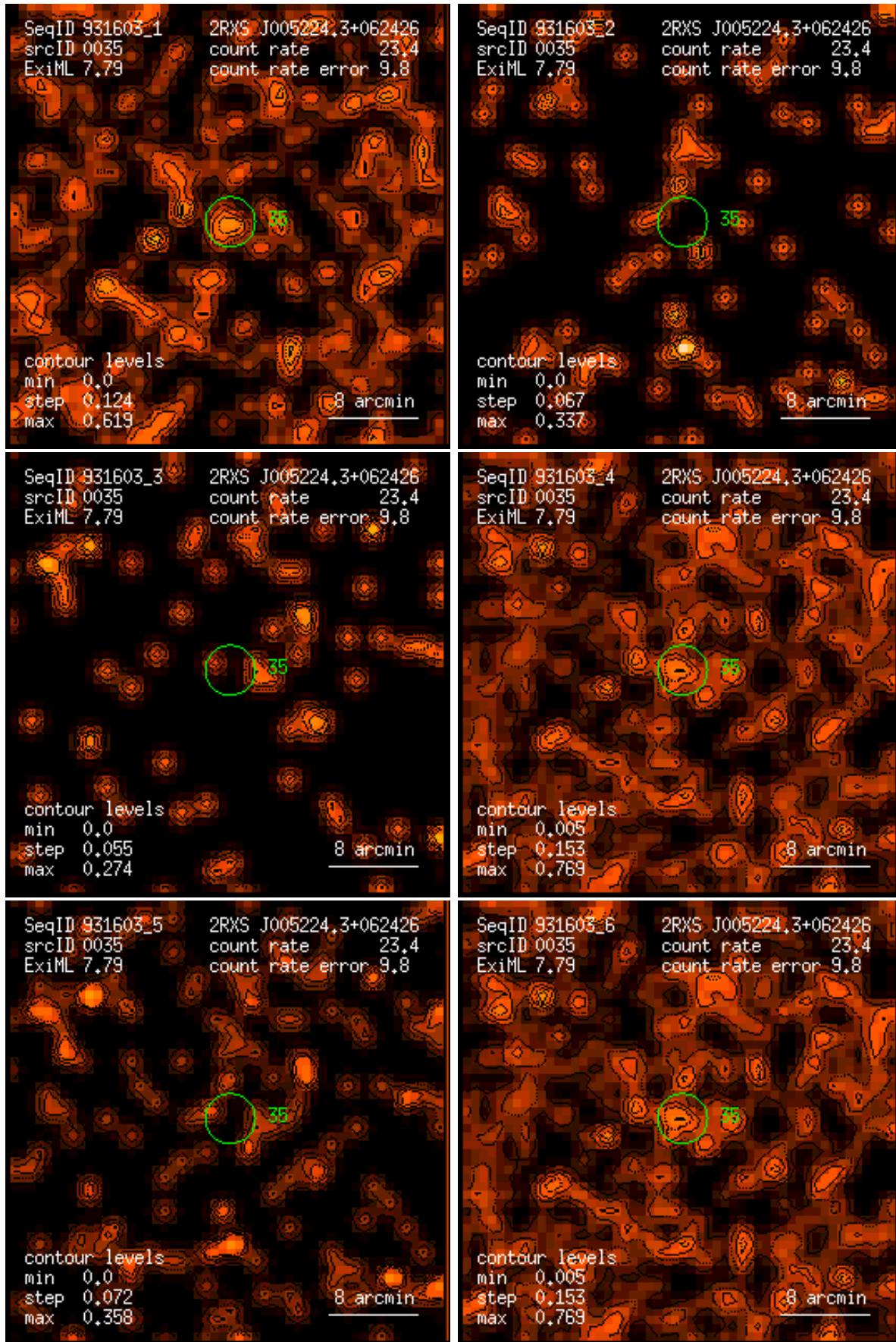
Figure 35: RASS 931603: detection 0035: band rate images, Gaussian filter: (1) PSPC channels 11 – 41, (2) 52 – 90, (3) 91 – 201, (4) 11 – 235, (5) 52 – 201, (6) 11 – 201. Broad band rates in counts/ks. Band rate contour levels in counts/ks/arcmin 2 .
