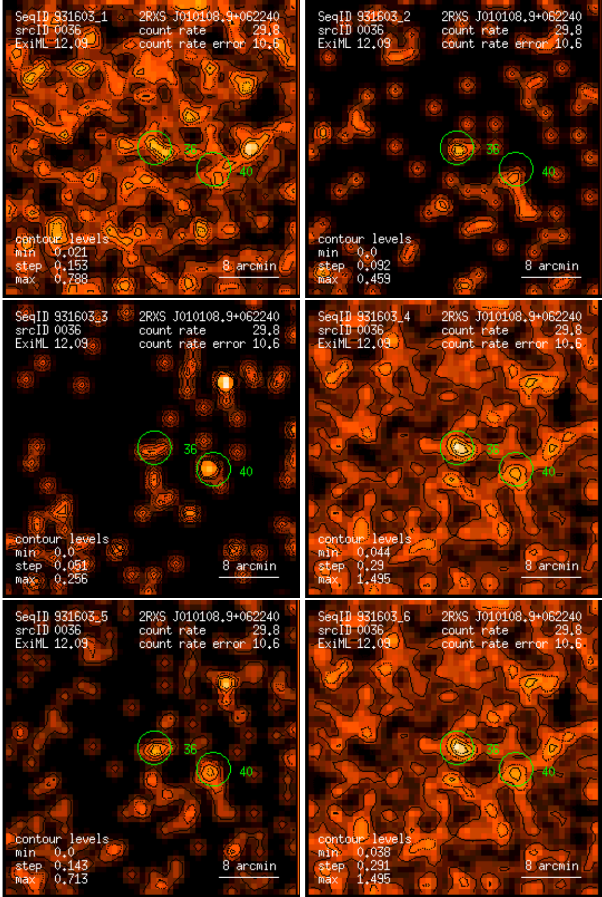
Figure 36: RASS 931603: detection 0036: band rate images, Gaussian filter: (1) PSPC channels 11 – 41, (2) 52 – 90, (3) 91 – 201, (4) 11 – 235, (5) 52 – 201, (6) 11 – 201. Broad band rates in counts/ks. Band rate contour levels in counts/ks/arcmin 2 .
