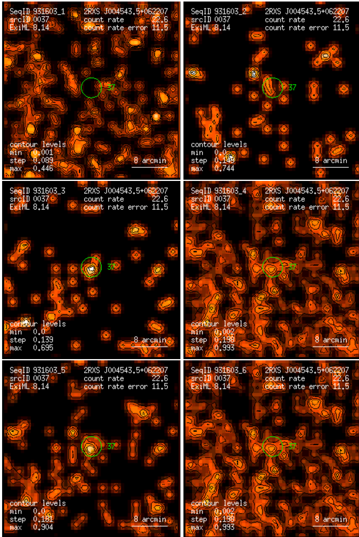
Figure 37: RASS 931603: detection 0037: band rate images, Gaussian filter: (1) PSPC channels 11 – 41, (2) 52 – 90, (3) 91 – 201, (4) 11 – 235, (5) 52 – 201, (6) 11 – 201. Broad band rates in counts/ks. Band rate contour levels in counts/ks/arcmin 2 .
